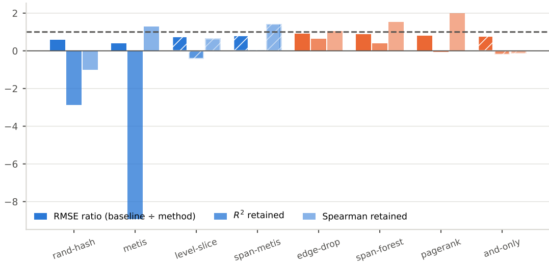
Accuracy retained under reduction (1.0 = no loss; below 0 = worse than the mean)
