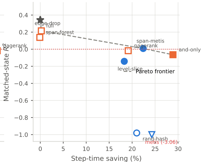
R^2 vs. Step-time saving (%)
