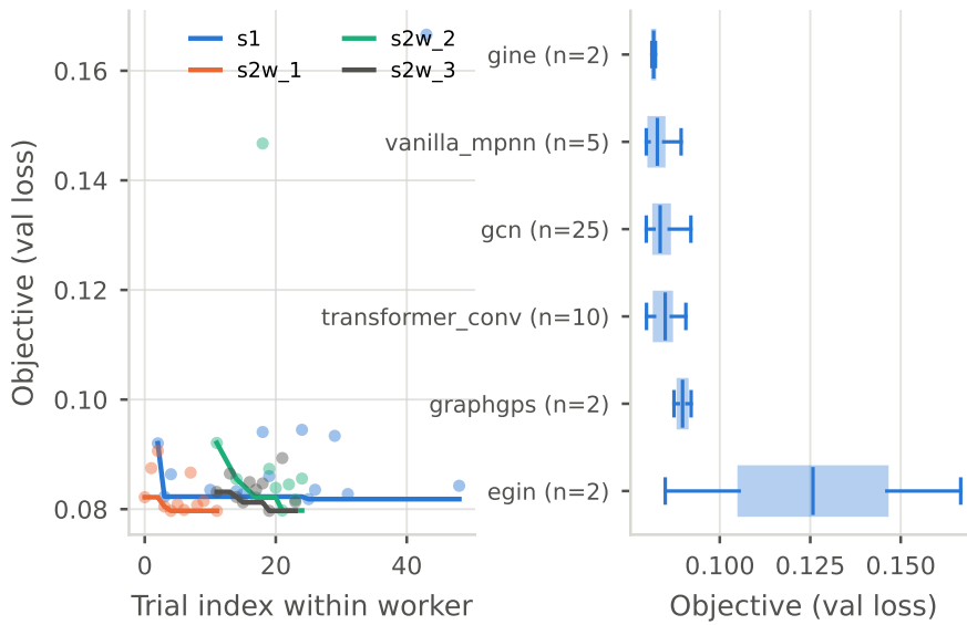
Sweep progress (6 outliers clipped) Objective by encoder
