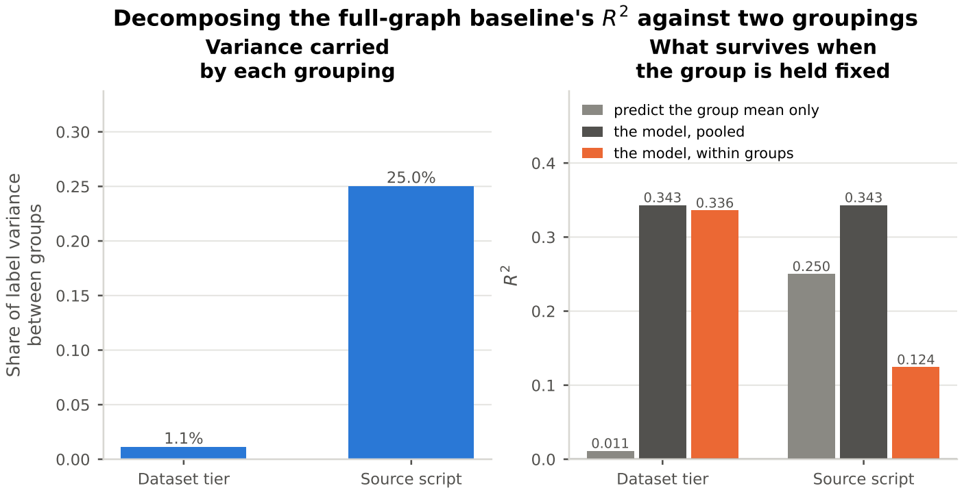
Figure 4.10: How much of the full-graph baseline's R^2 = 0.343 is reachable without learning anything about an individual circuit. Grouping by dataset tier carries only 1.1% of the label variance, so the tier is not a confound. Grouping by source script carries 25.0%: a predictor that outputs nothing but each group's mean scores R^2 = 0.250 , i.e. roughly three-quarters of the model's reported figure. Held against within-group variance the model retains R^2 = 0.124 . That residual is the part attributable to reading circuit structure, and it is the number 4.1 should defend.
