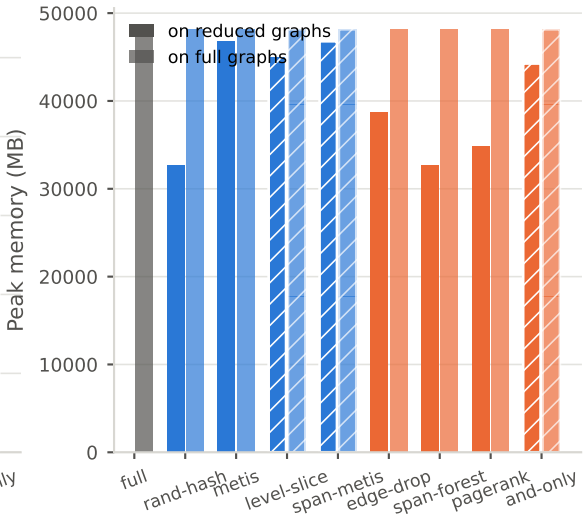
Inference peak memory
