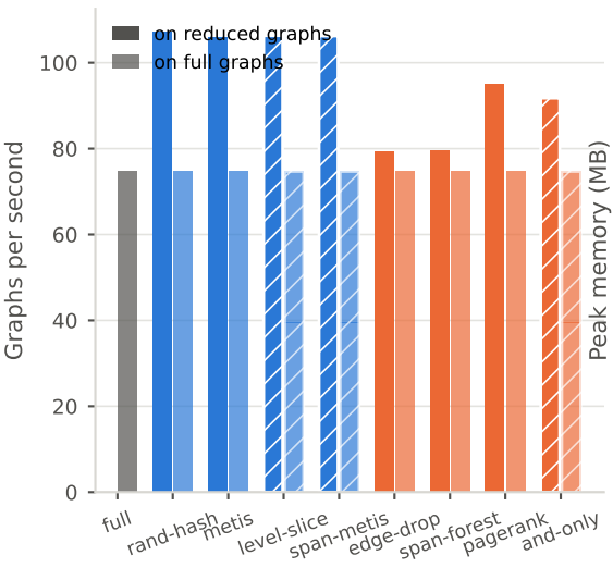
Inference throughput
