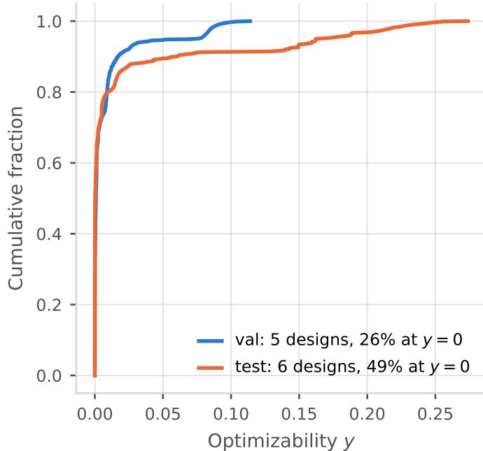
Figure 3.8: Validation and test are disjoint circuit sets, not exchangeable samples: 26% of validation graphs sit at y = 0 against 49% of test, and the test maximum y is more than twice the validation maximum. This is expected under a design-level split (3.4.2) and is the direct explanation for the validation-to-test gap in 4.37; it also bounds how much validation-based model selection can be assumed to transfer.
