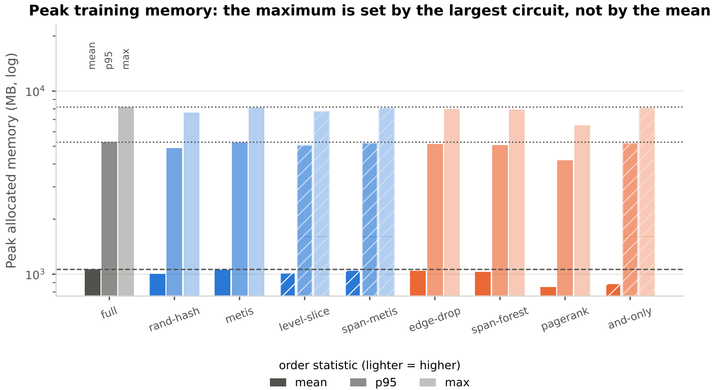
Figure 4.21: Peak allocated device memory per configuration at three order statistics. The mean, p95 and maximum disagree by an order of magnitude: a graph larger than the batch budget forms a batch of its own, so the maximum is floored by the largest circuit in the corpus no matter what the reduction did to the average one.
