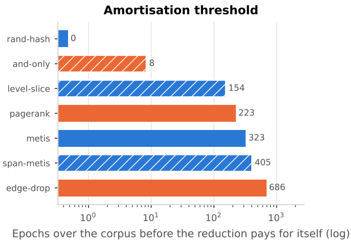
Figure 4.18: How many epochs over the corpus a cached reduction must serve before its offline cost is repaid by the training time it saves. This is the form in which 3.4.3 asks offline cost to be reported.
