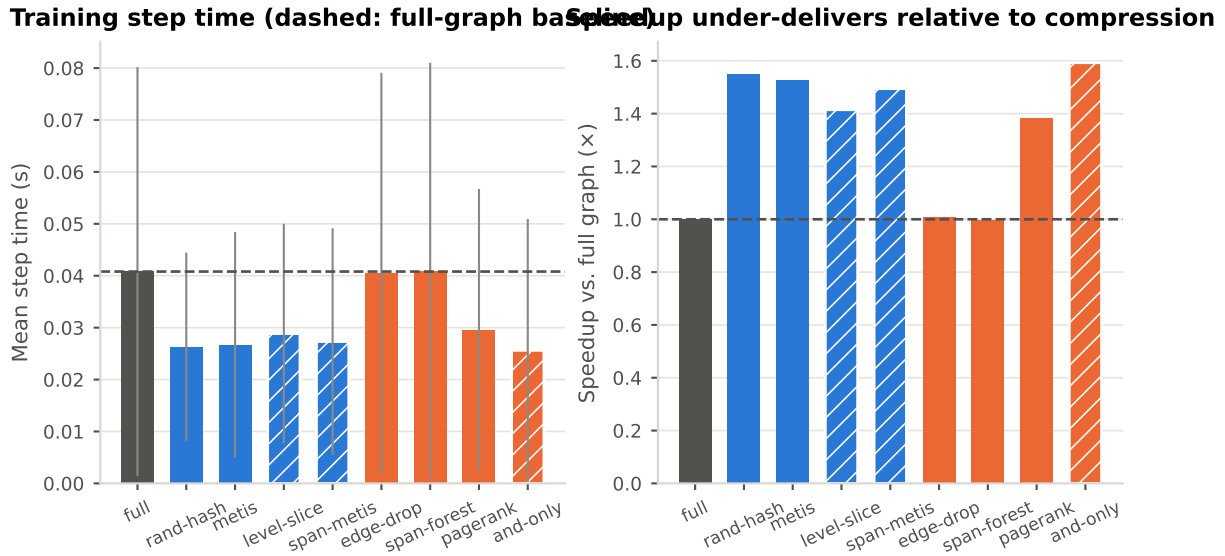
Figure 4.23: Mean step time and speedup against the full-graph baseline. Speedup under-delivers relative to compression, because the kernels are latency-bound on message-passing gather and scatter (3.4.2), so removing work does not translate proportionally into wall-clock time.
