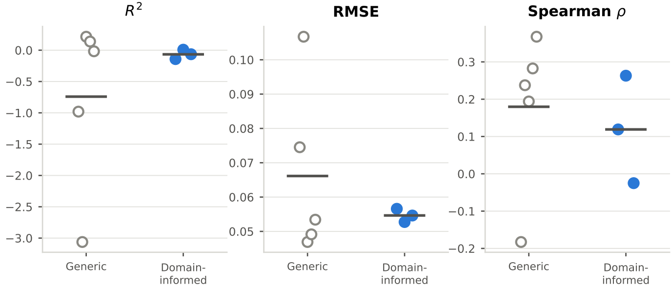
Figure 4.39: Every domain-informed method against every generic one on the same axes. Weaker evidence than the pairings, since the two groups did not remove the same amount, but it answers the question a reader asks first.
