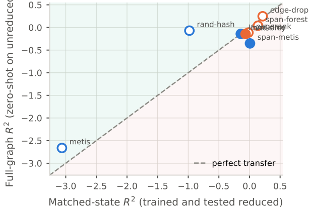
Figure 4.46: Matched-state against full-graph R^2 . The diagonal is perfect transfer. Below it the structural shift cost accuracy, above it the reduction was the thing doing damage.
