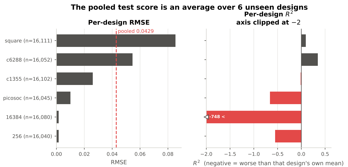
Figure 4.9: Per-design RMSE and R^2 for the full-graph baseline on the design-disjoint test set. The spread across designs is very wide and R^2 is strongly negative on some of them.
