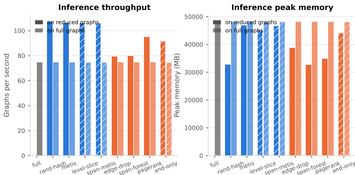
Figure 4.48: Throughput and peak memory for a query, under each evaluation state. Inference stores neither gradients nor activations, so the memory argument that forced the reduction at training time need not bind here at all, which is the practical claim of 1.2.5.
