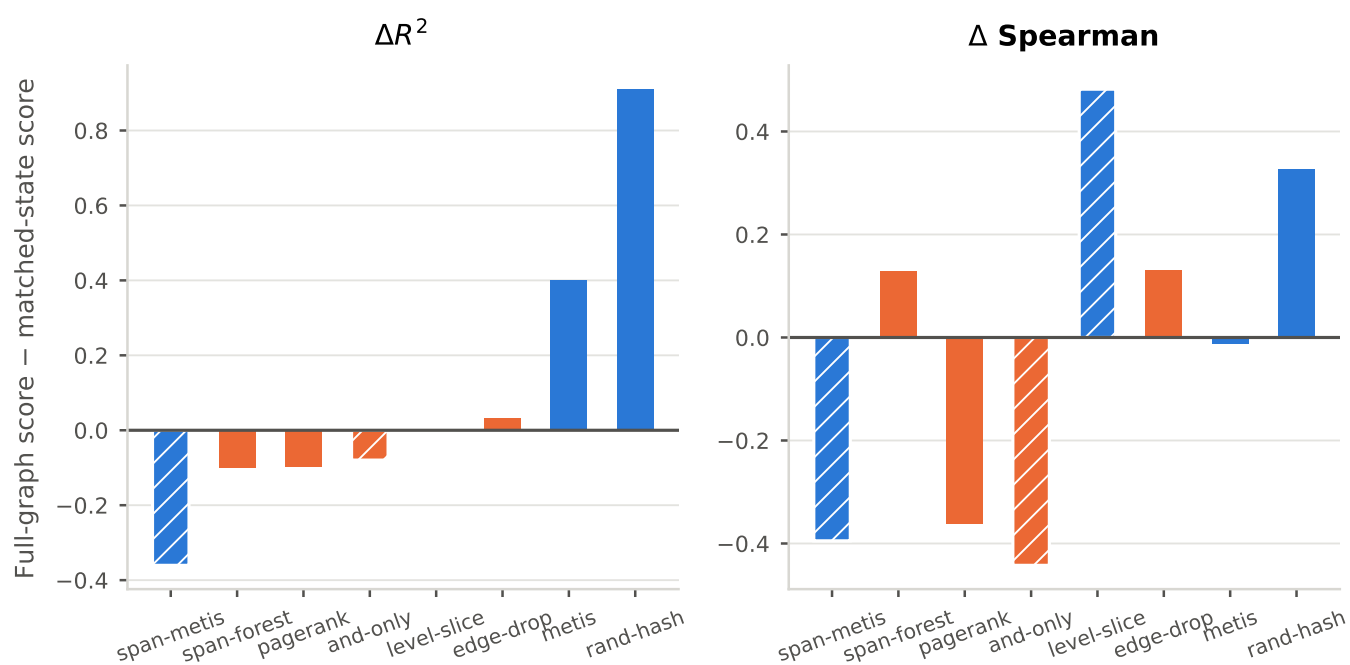
Figure 4.47: Full-graph score minus matched-state score, by method and family. A positive bar means the model scores better on graphs it never trained on, which would say the reduction was hurting the model rather than the evaluation.
