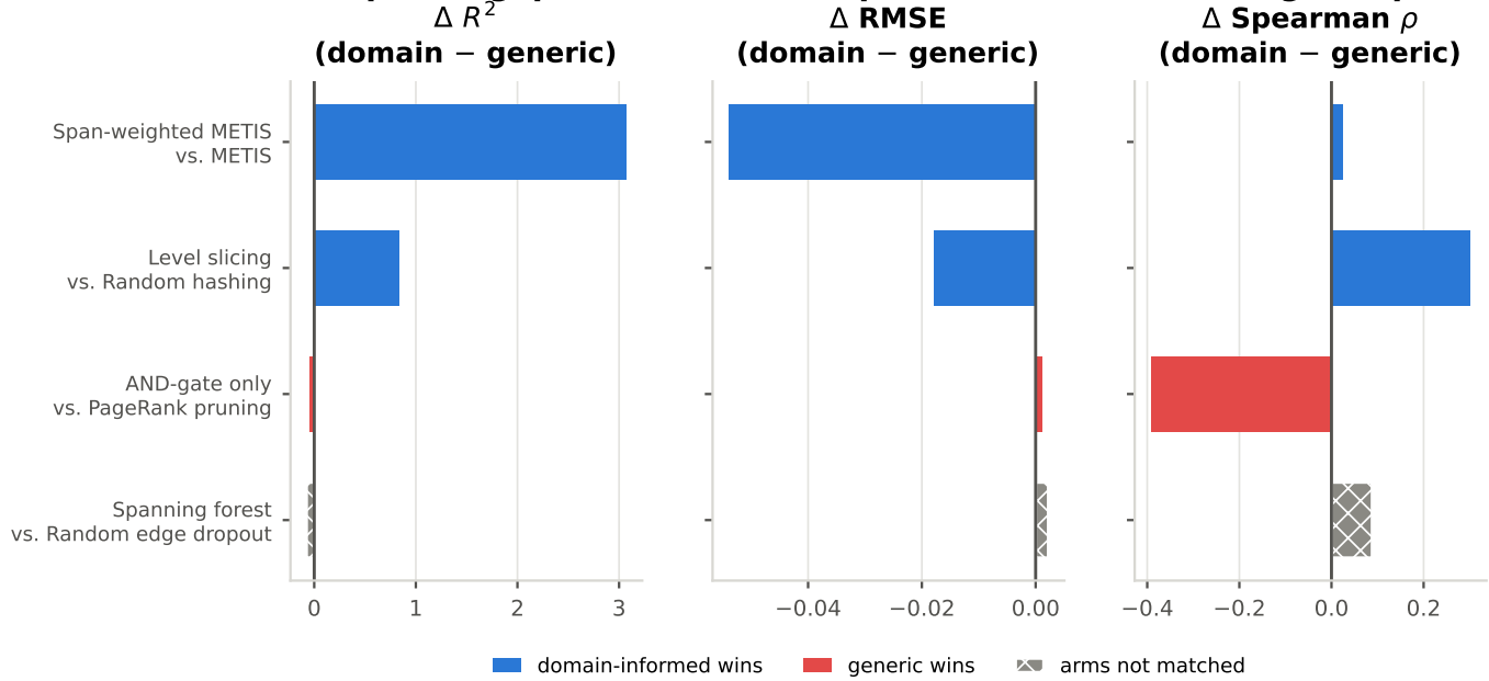
Figure 4.40: Domain-informed minus generic within each pairing. The first two pairings are matched by construction (same k , all nodes kept, only the cut rule differs). The third is matched by calibration. The fourth is not matched and is hatched accordingly. Read every bar against 4.38.
