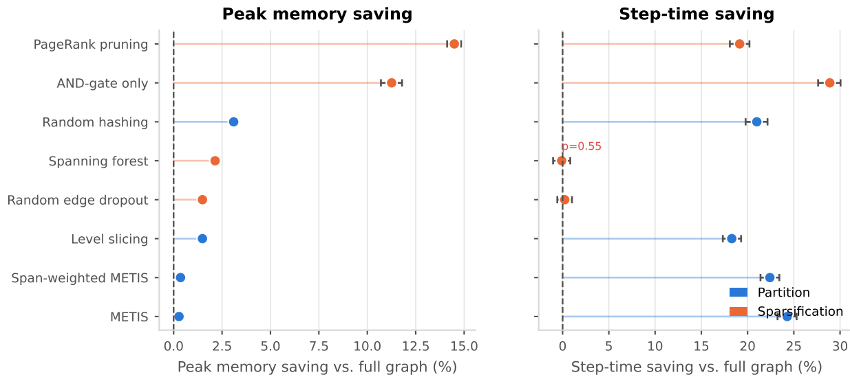
Figure 4.24: Per-graph peak-memory and step-time savings against the baseline, paired by graph id, with 95% percentile bootstrap intervals. A red p -value marks a Wilcoxon signed-rank test that fails to separate the saving from noise.
