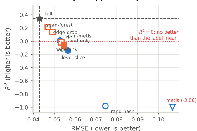
Figure 4.26: RMSE against R^2 , one point per configuration. Several configurations hold RMSE close to the baseline while R^2 falls below zero, which is the same dissociation Khadka et al. [2026] report on a coarsened EDA graph.
