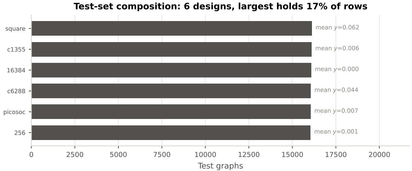
Figure 3.7: How the design-disjoint test set is composed. Under a design-level split the test set is a handful of whole circuits rather than a random sample, so every pooled test metric is an average over these designs and their mix.
