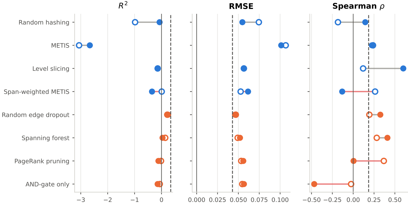
Figure 4.44: The same weights evaluated under the reduction they were trained with and on unreduced graphs. For every method here a full graph needs no conversion, since it already is a valid input, which is what makes this a direct test rather than a comparison across two input formats (3.2.3).
