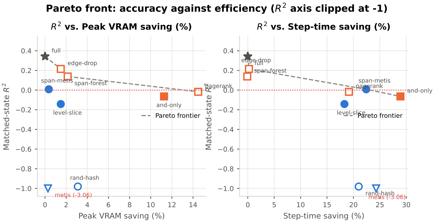
Figure 4.26: Accuracy against efficiency, with the dominance frontier drawn. The full-graph baseline sits on the same axes at zero saving, so “no reduction” competes directly against every reduction.
