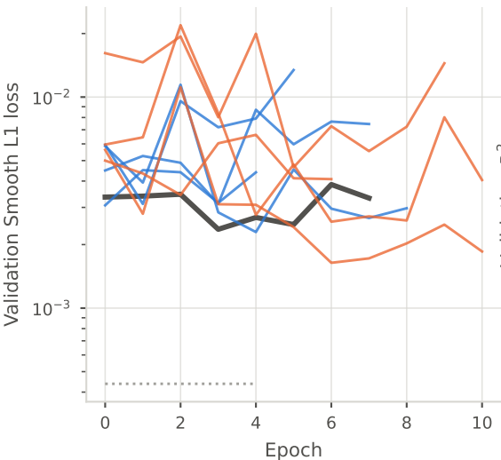
Validation loss
