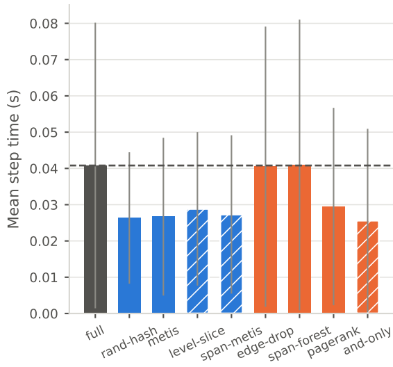
Training step time (dashed: full-graph baseline) Speedup under-delivers relative to compression
