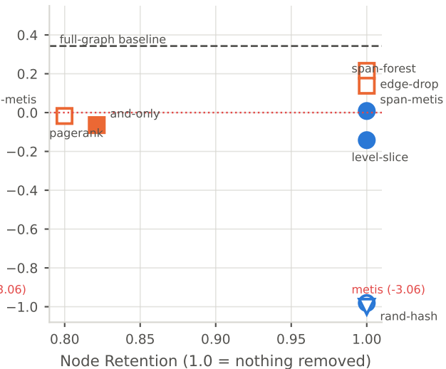
R^2 vs. node retention
