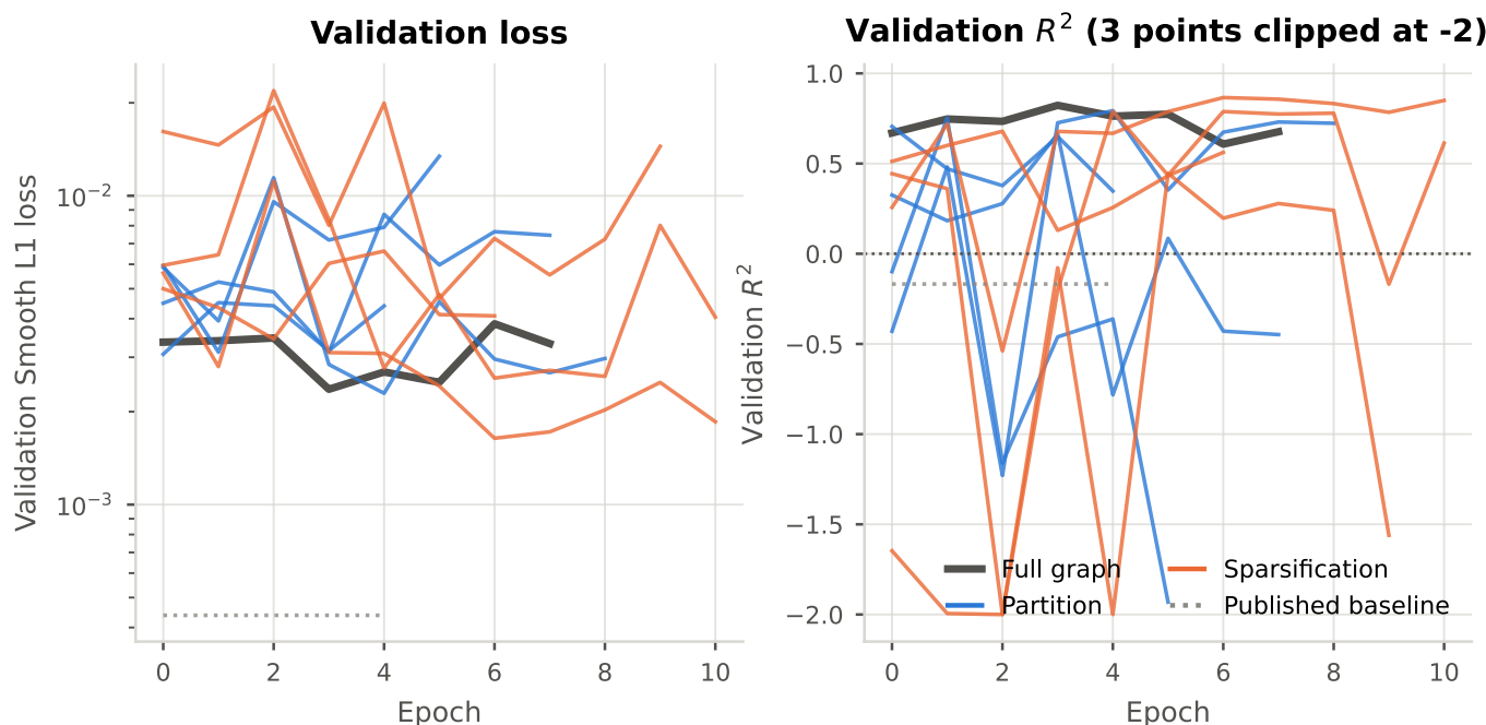
Figure 4.7: Validation loss and R^2 per epoch for every Orchestrate training run, coloured by reduction family. Validation R^2 swings by several units between consecutive epochs on some configurations, which bounds how much weight any single-seed comparison can carry (3.4.3).
