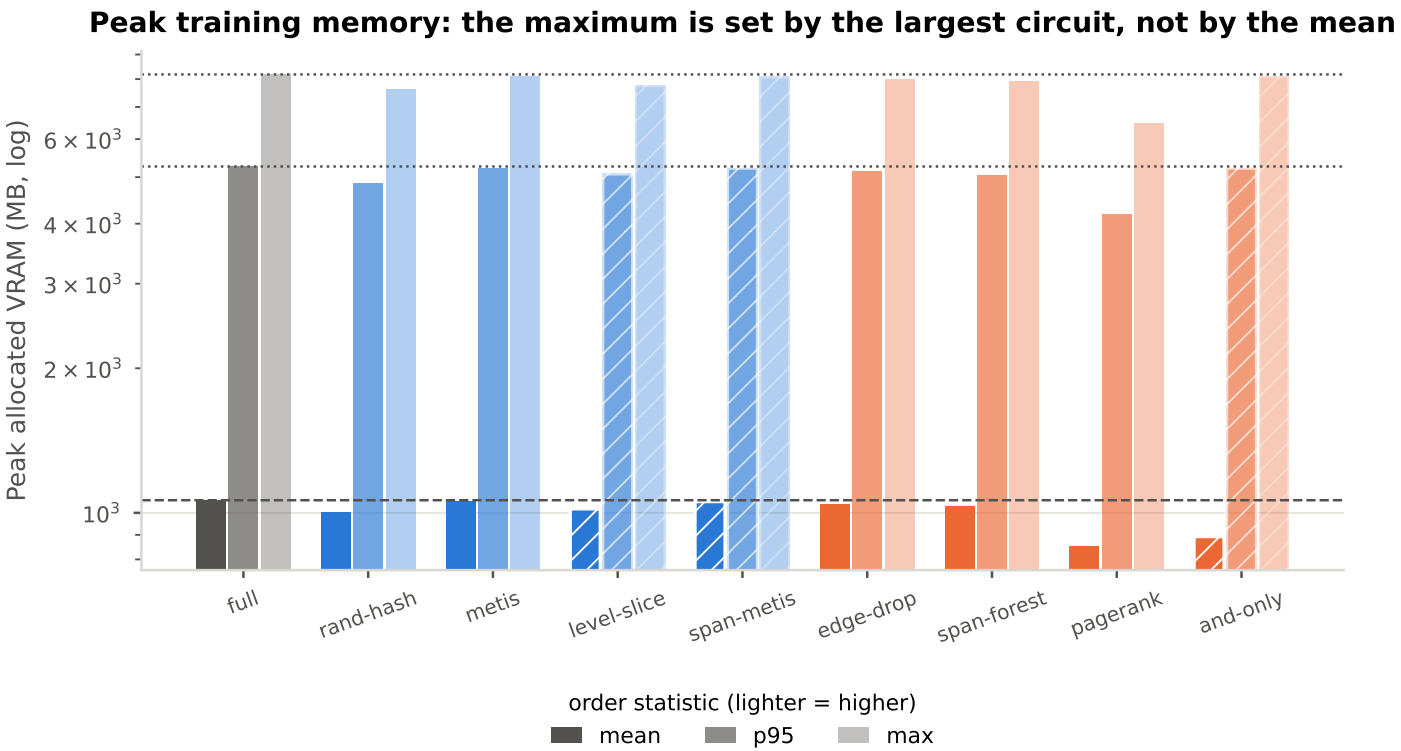
Figure 4.18: Peak allocated device memory per configuration at three order statistics. The mean, p95 and max disagree by an order of magnitude, and that gap is the point: a graph larger than the batch budget forms a batch of its own, so the maximum is floored by the largest circuit in the corpus no matter what the reduction did to the average one.
