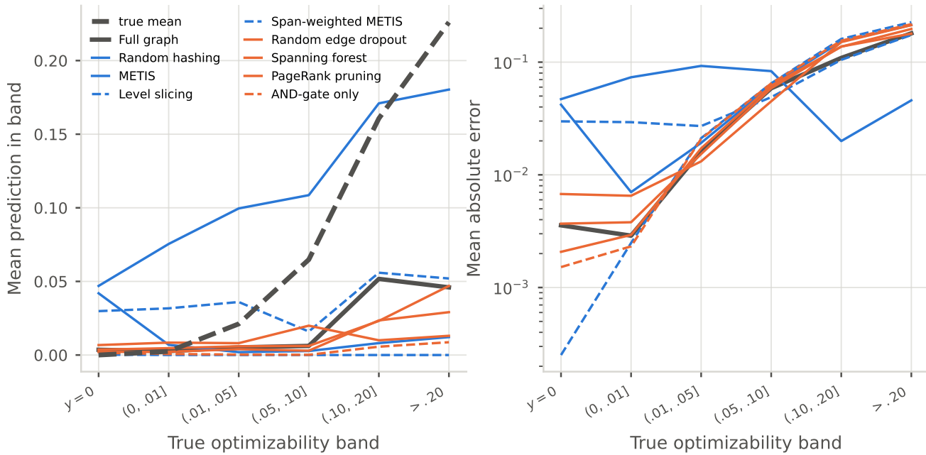
Figure 4.33: Every configuration as a function of how optimizable the circuit truly is. Level slicing predicts 0.0000 in every band, a fully collapsed model that the pooled metrics do not expose. METIS over-predicts everywhere, which is why its pooled R^2 is -3.06 , yet that same miscalibration makes it the most accurate configuration on the highly optimizable circuits: MAE 0.046 above y = 0.20 against the unreduced baseline's 0.180.
