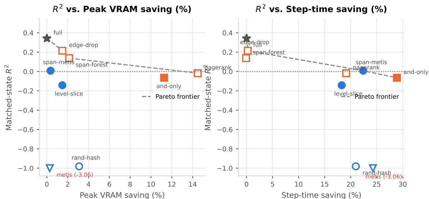
Figure 4.36: Accuracy against efficiency, with the dominance frontier drawn. The full-graph baseline sits on the same axes at zero saving, so “no reduction” competes directly against every reduction rather than sitting outside the comparison.
