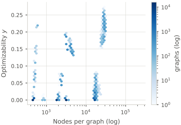
Size vs. label (Spearman \rho = 0.166 )
