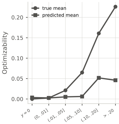
Prediction against truth by band
