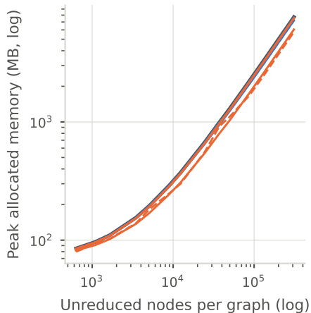
Absolute memory: every method traces one curve
