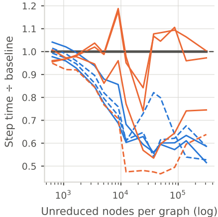
Step time relative to the full graph
