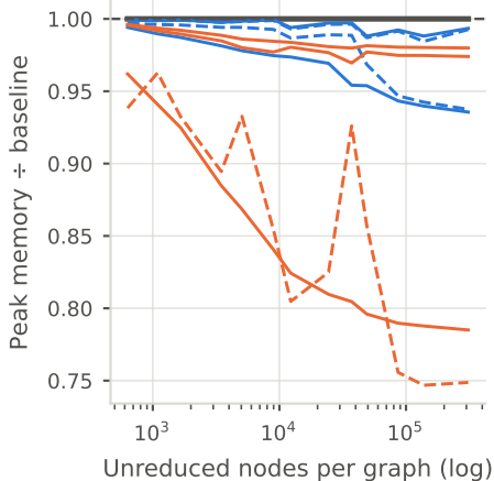
Memory relative to the full graph
