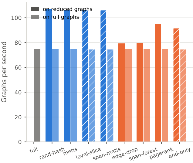
Inference throughput
