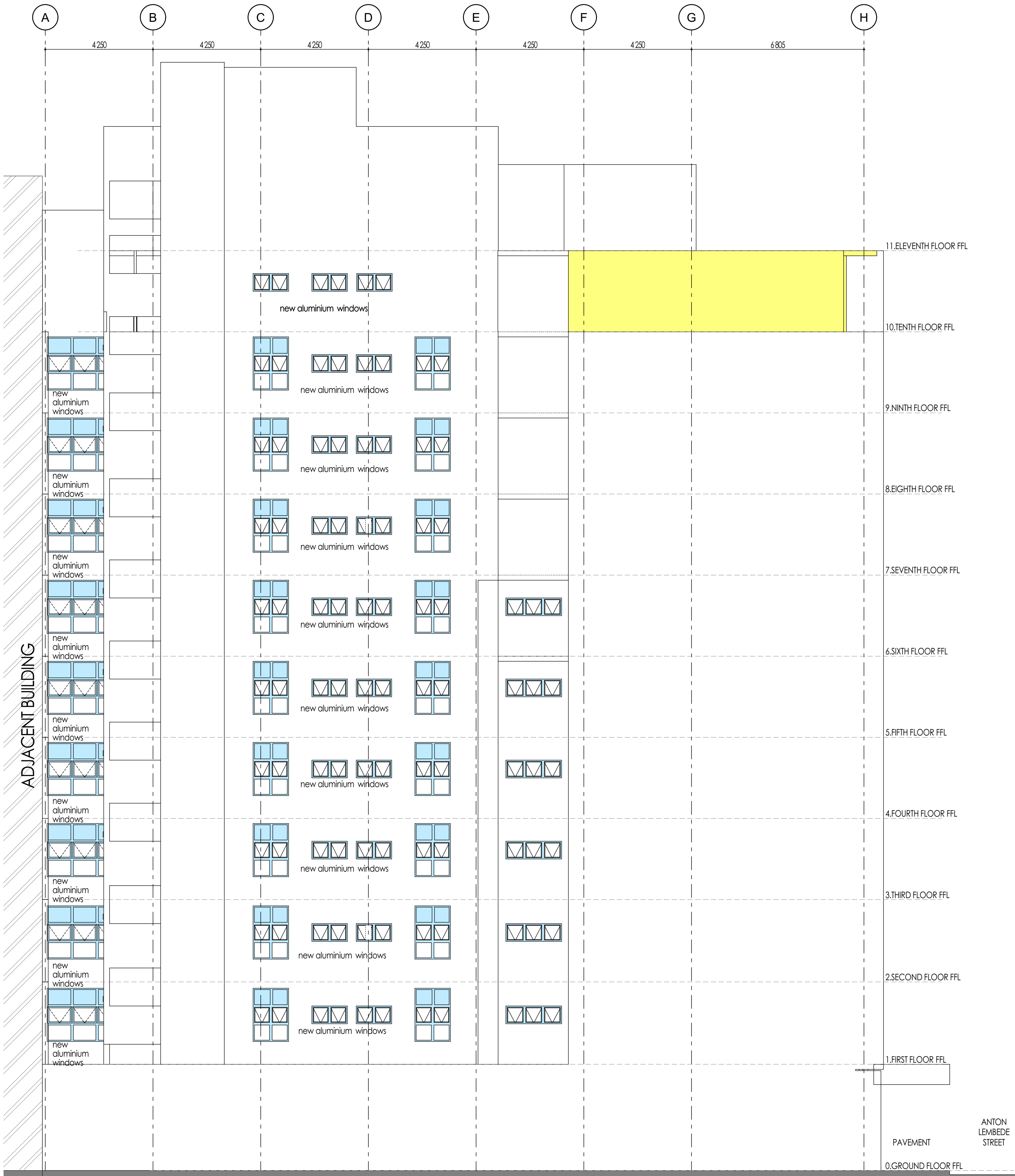
EAST ELEVATION SCALE 1:100
