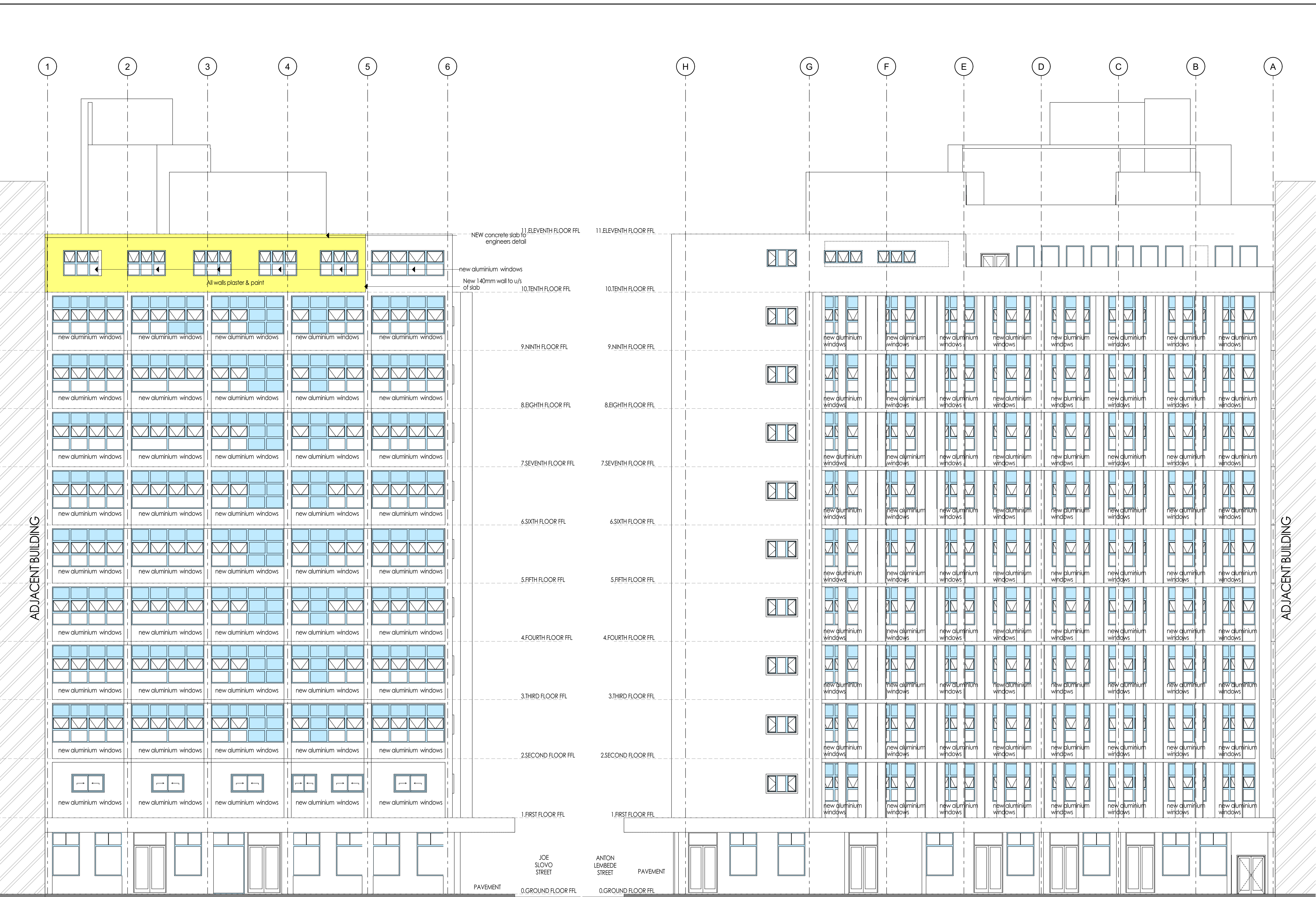
NORTH ELEVATION SCALE 1:100 WEST ELEVATION SCALE 1:100
