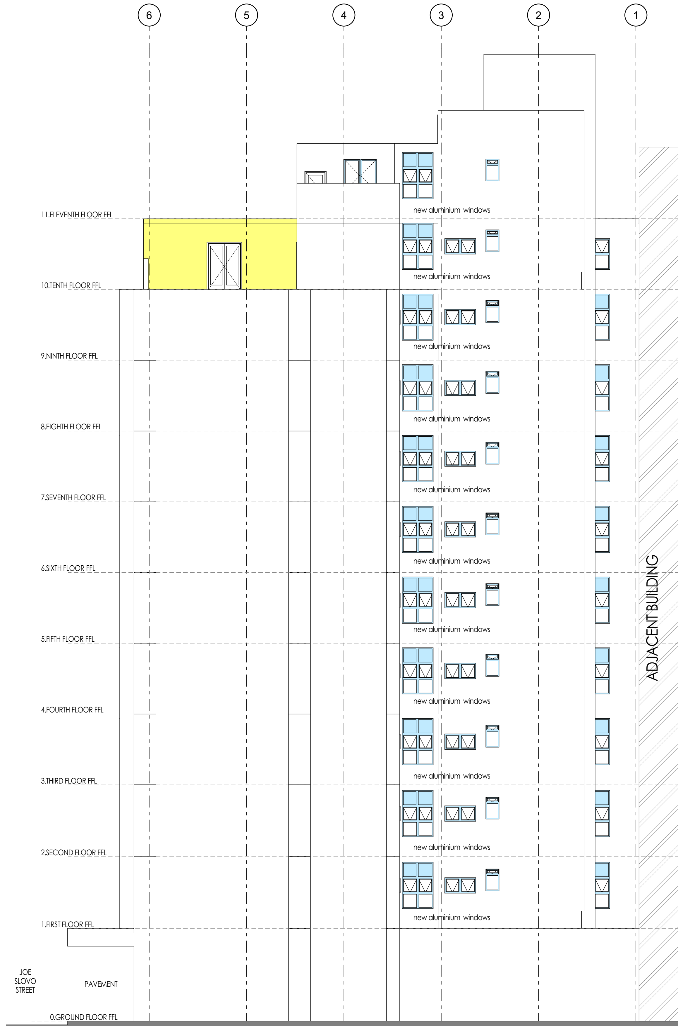
SOUTH ELEVATION SCALE 1:100
