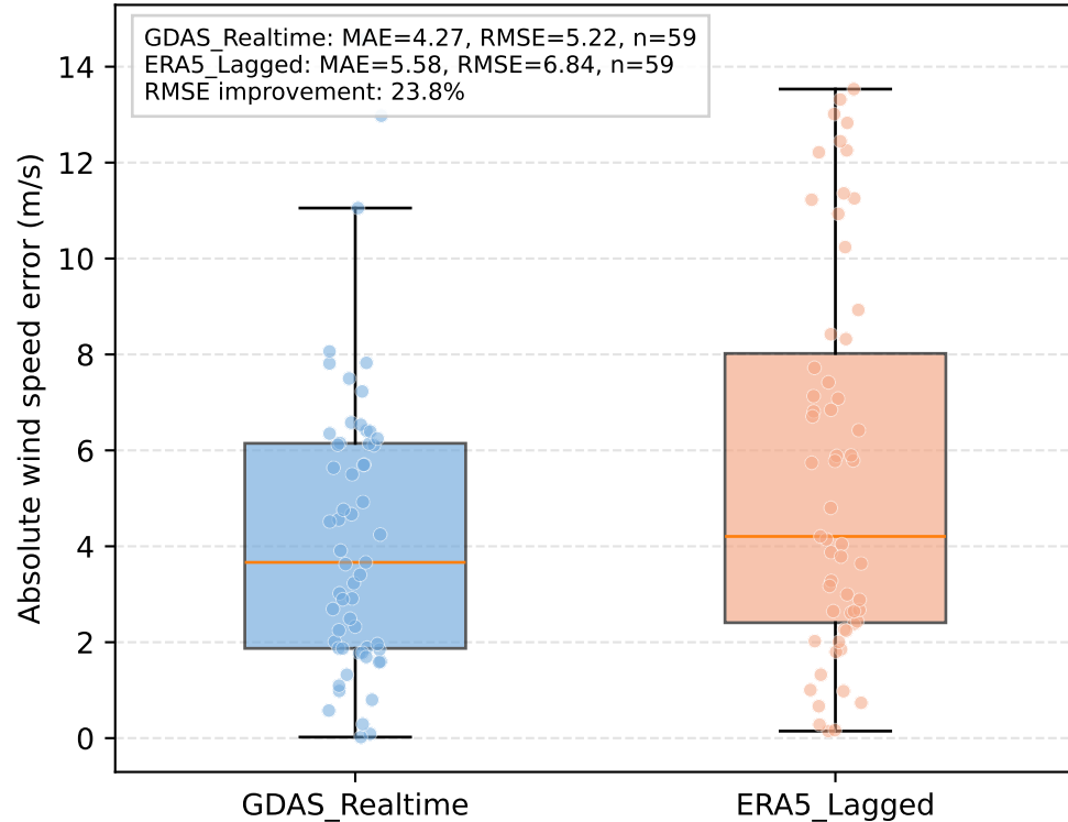
(b) Absolute wind speed error
