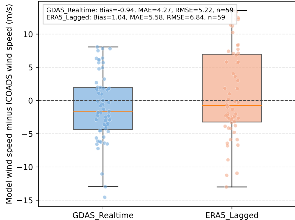
(a) Wind speed error
