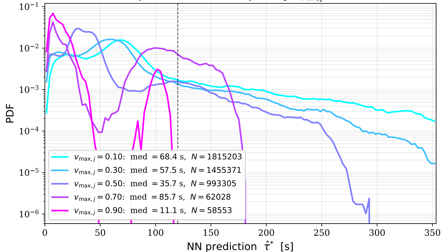
NN predictions on Inf inputs by v_{\max,j} (vraw)
