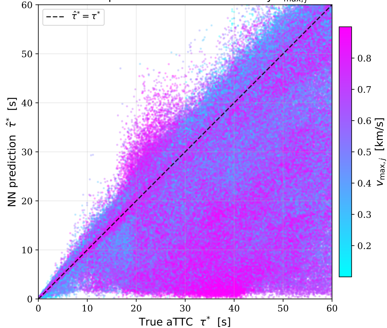
True vs predicted aTTC — colored by v_{\max,j}
