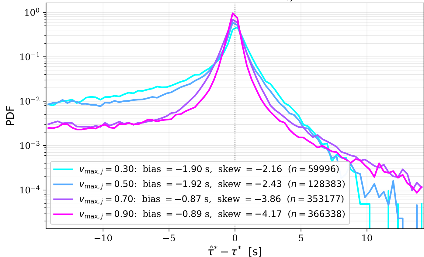
Signed prediction error by v_{\max,j} ( \tau^* < 30 s)
