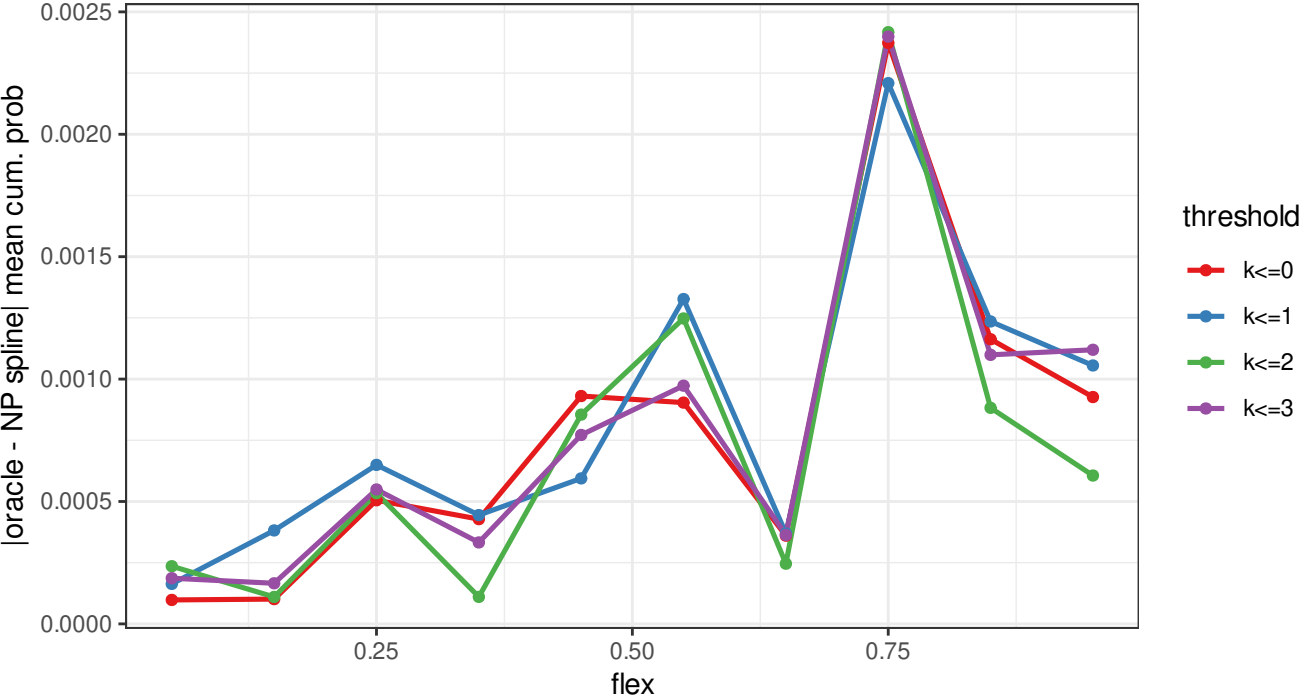
D: |\text{oracle mean } P(X \leq k) - \text{NP spline mean } P(X \leq k)|
