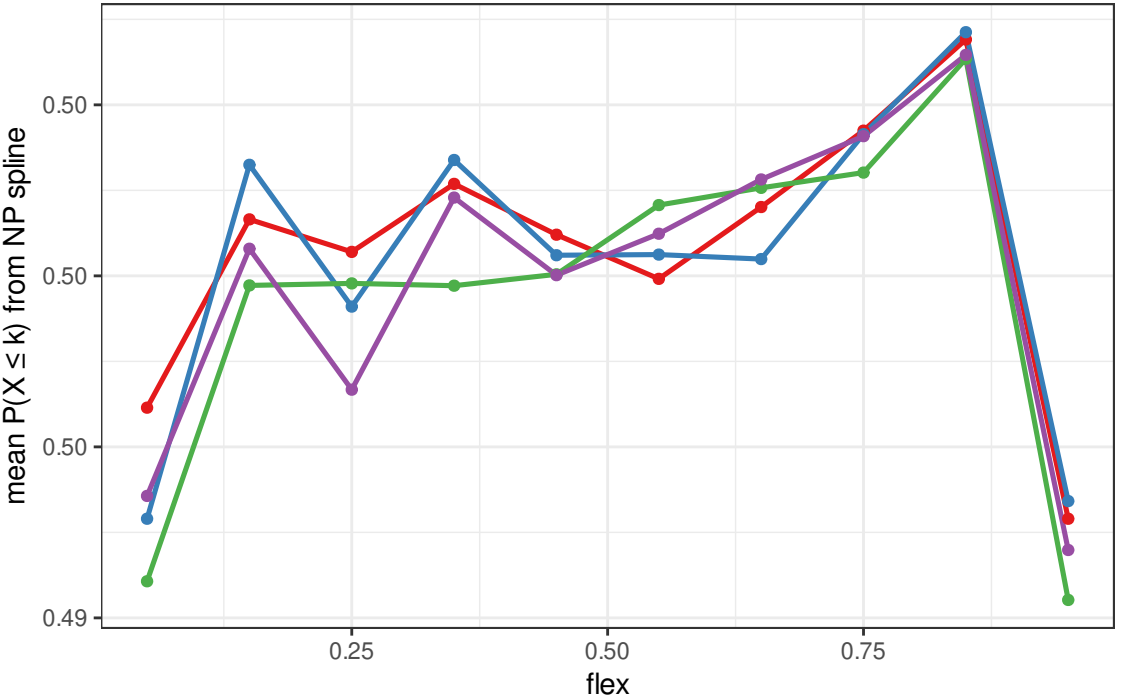
C: mean NP spline cumulative probability P(X \leq k)
