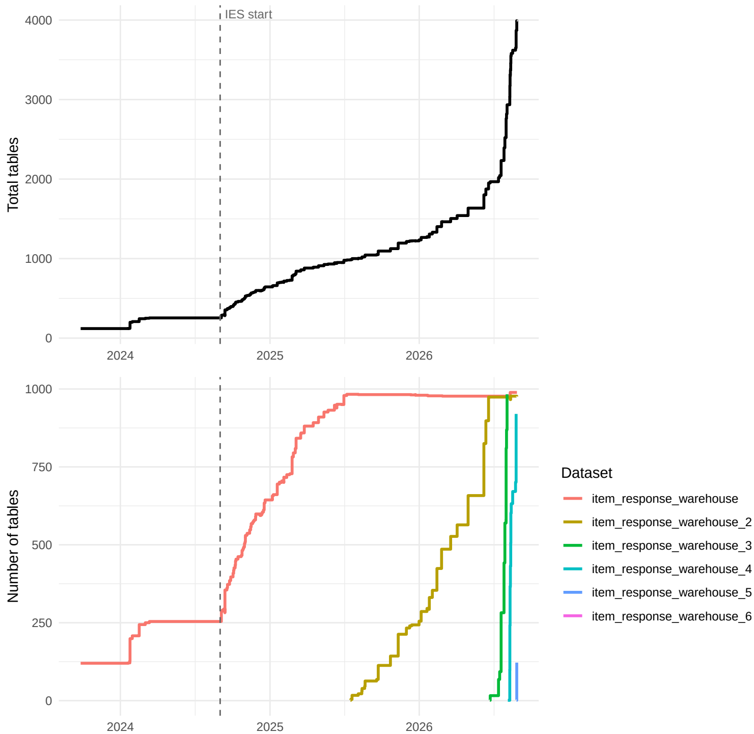
Growth of the IRW core datasets
