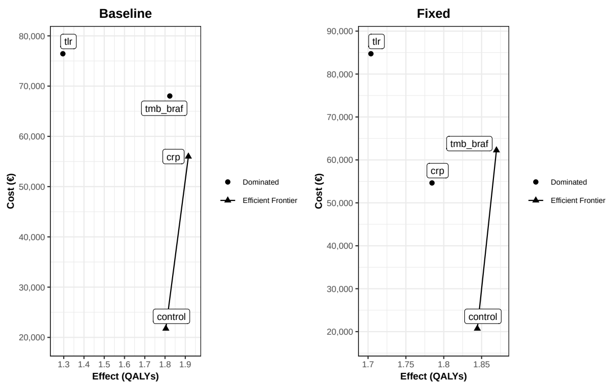
Figure 1: Cost-effectiveness efficiency frontier comparison using dampack. Baseline (left) and fixed (right) strategies are shown with the efficiency frontier connecting non-dominated strategies. Dominated strategies appear off the frontier line.
