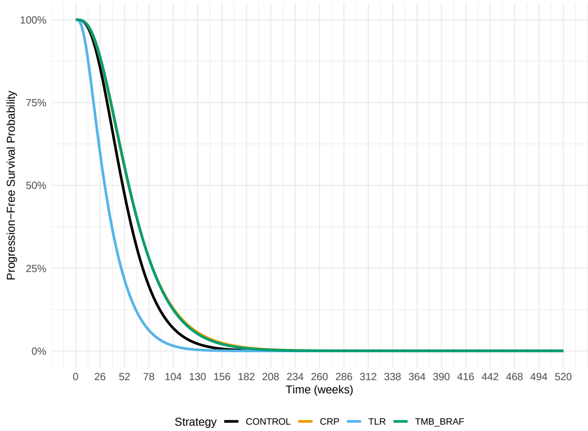
Figure 5: Progression-free survival comparison across all treatment strategies. Each curve represents the population-weighted expected PFS for each strategy: Control (standard of care for all patients), CRP-guided treatment allocation, TLR-guided treatment allocation, and TMB_BRAF-guided treatment allocation. Differences between strategies reflect both the predictive accuracy of each biomarker and its prevalence in the population.
