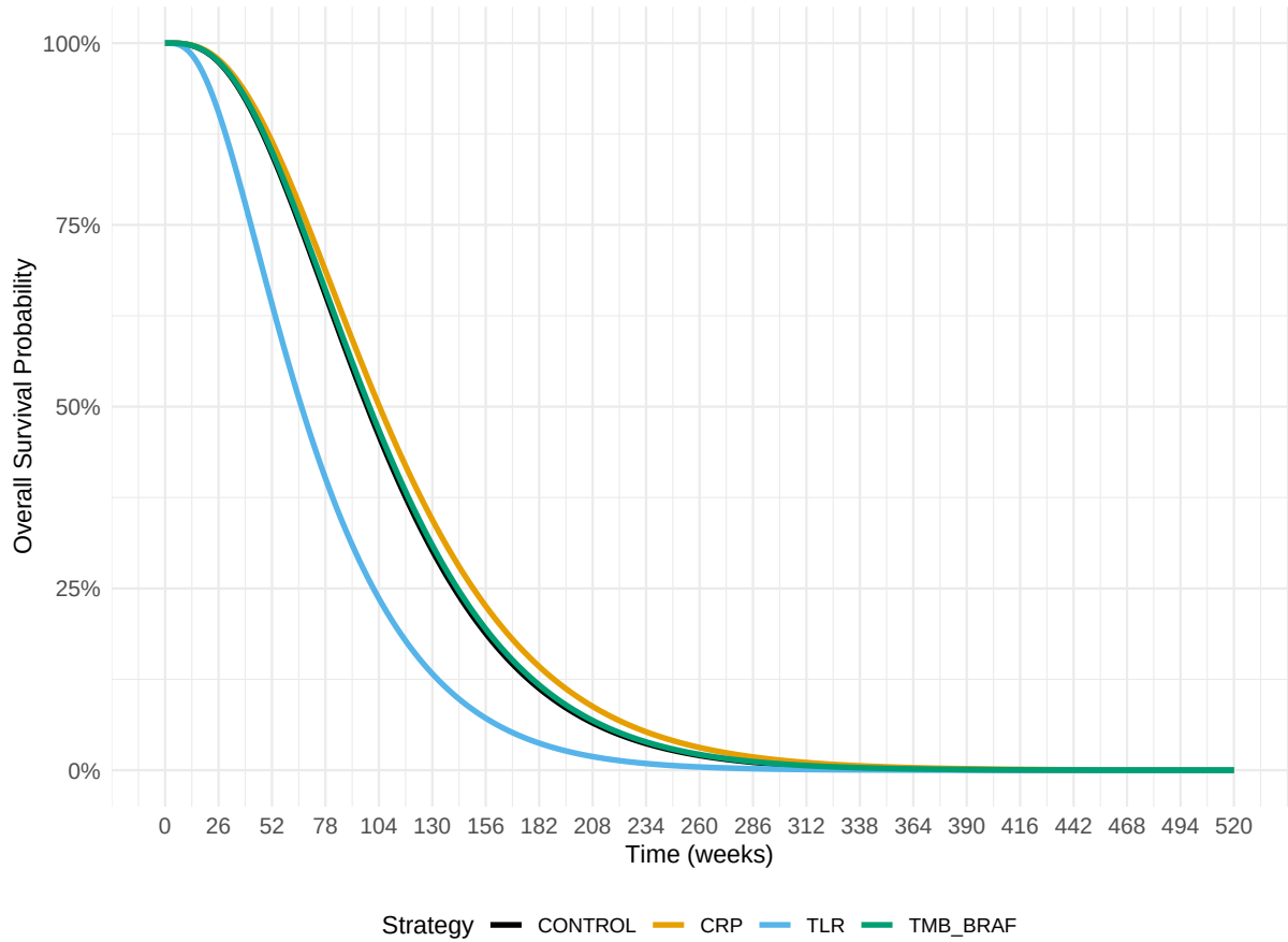
Figure 4: Overall survival comparison across all treatment strategies. Each curve represents the population-weighted expected OS for each strategy: Control (standard of care for all patients), CRP-guided treatment allocation, TLR-guided treatment allocation, and TMB_BRAF-guided treatment allocation. Differences between strategies reflect both the predictive accuracy of each biomarker and its prevalence in the population.
