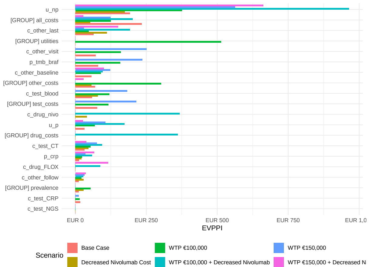
Figure 1: Scenario EVPPI by parameter
