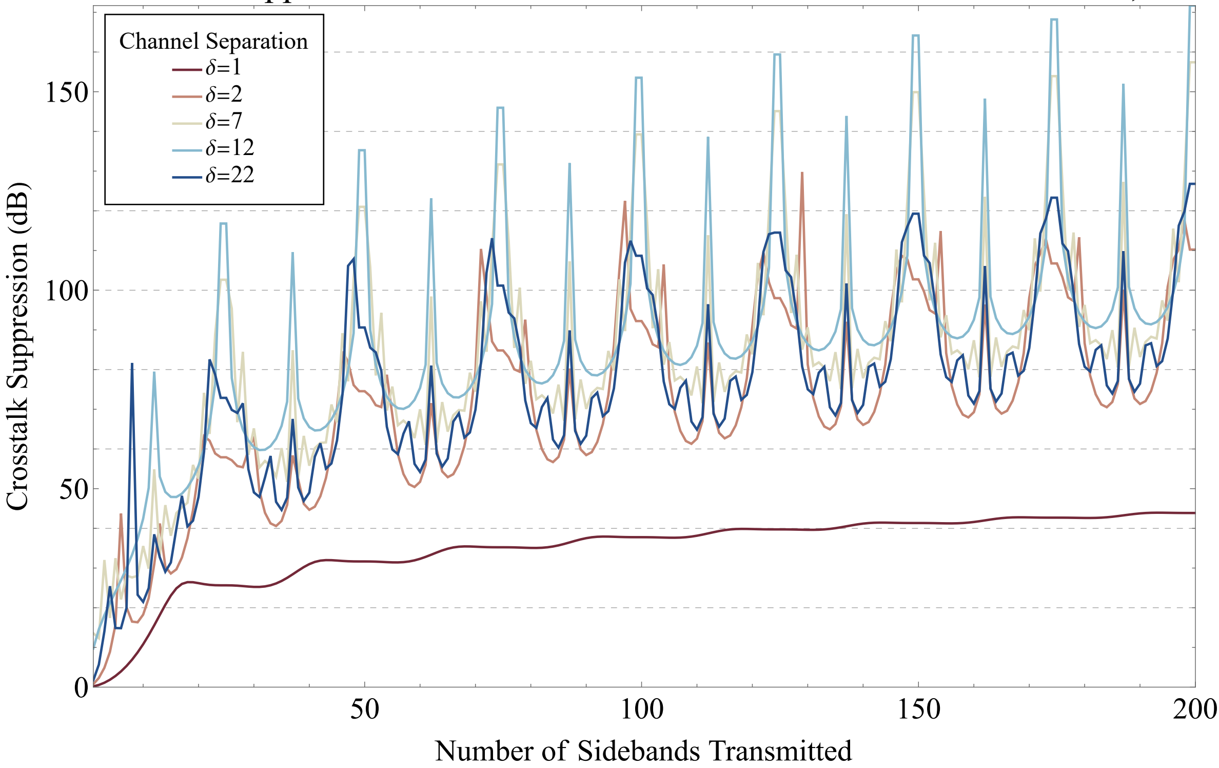
Crosstalk Suppression vs Transmission Line Bandwidth for 25 Channels, x=1
