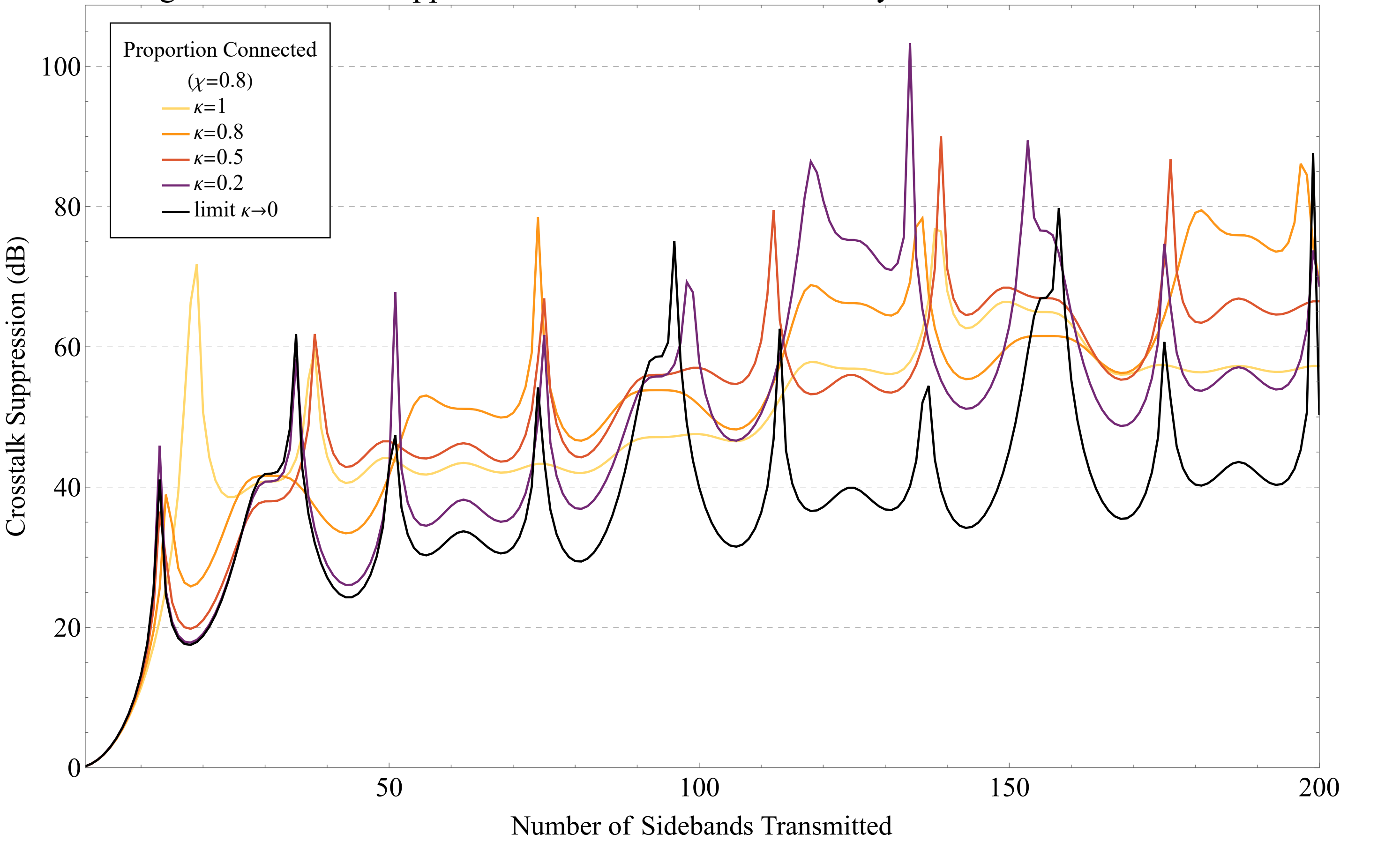
Nearest Neighbor Crosstalk Suppression for a 25 Channel TDM System vs Transmission Line Bandwidth
