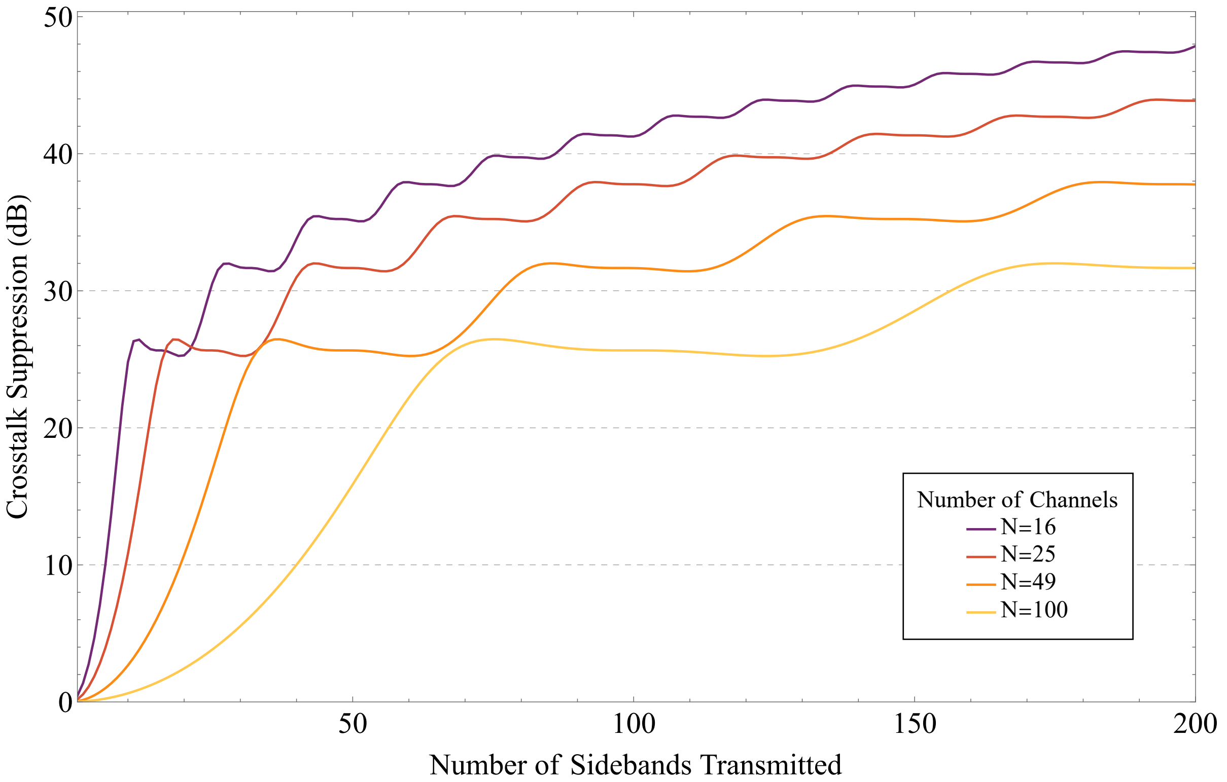
Nearest Neighbor Crosstalk Suppression vs Transmission Line Bandwidth for x=1
