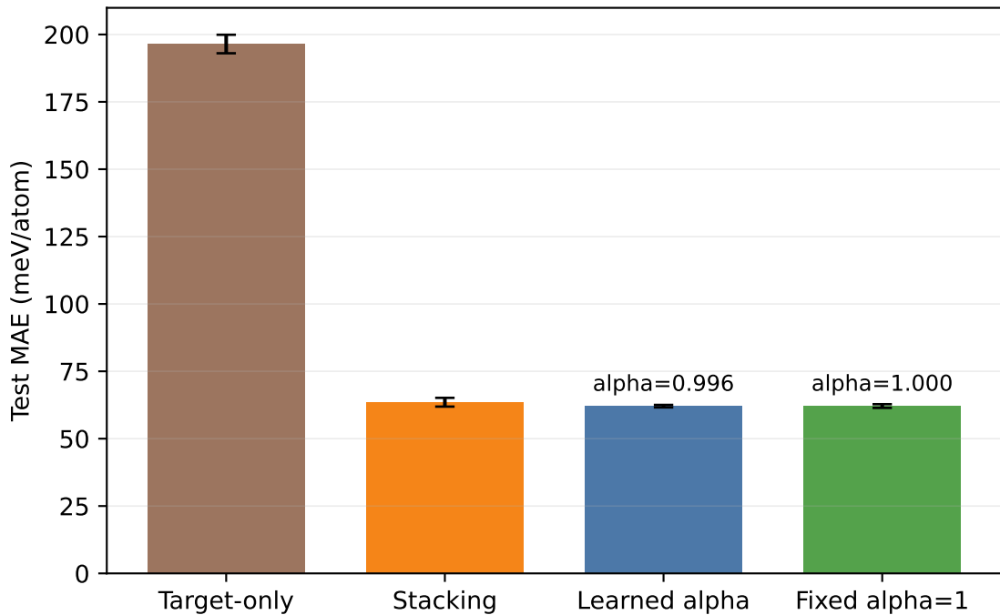
Current-recipe anchor ablation
