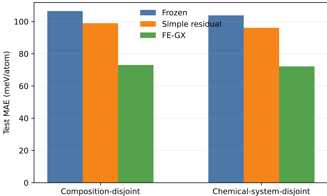
OOD generalization on the MEGNet target
