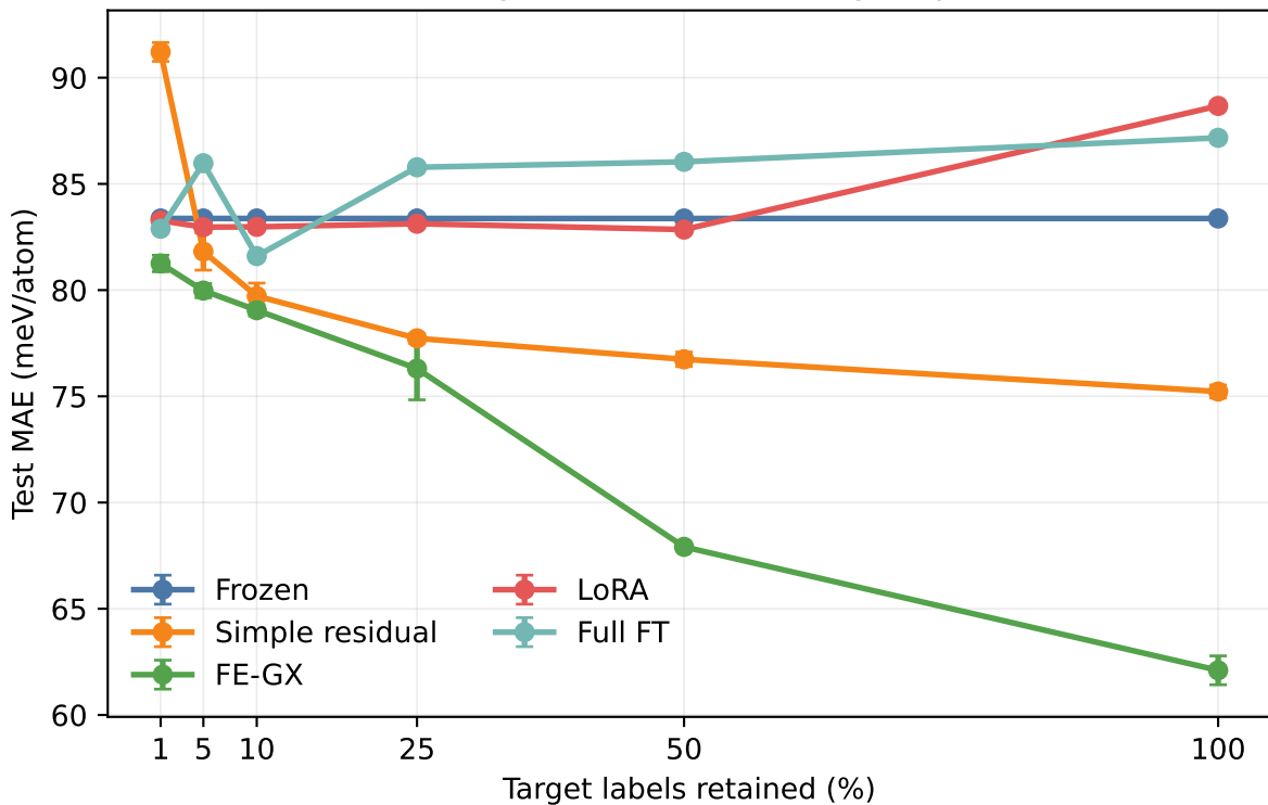
Scaling on the MEGNet target split
