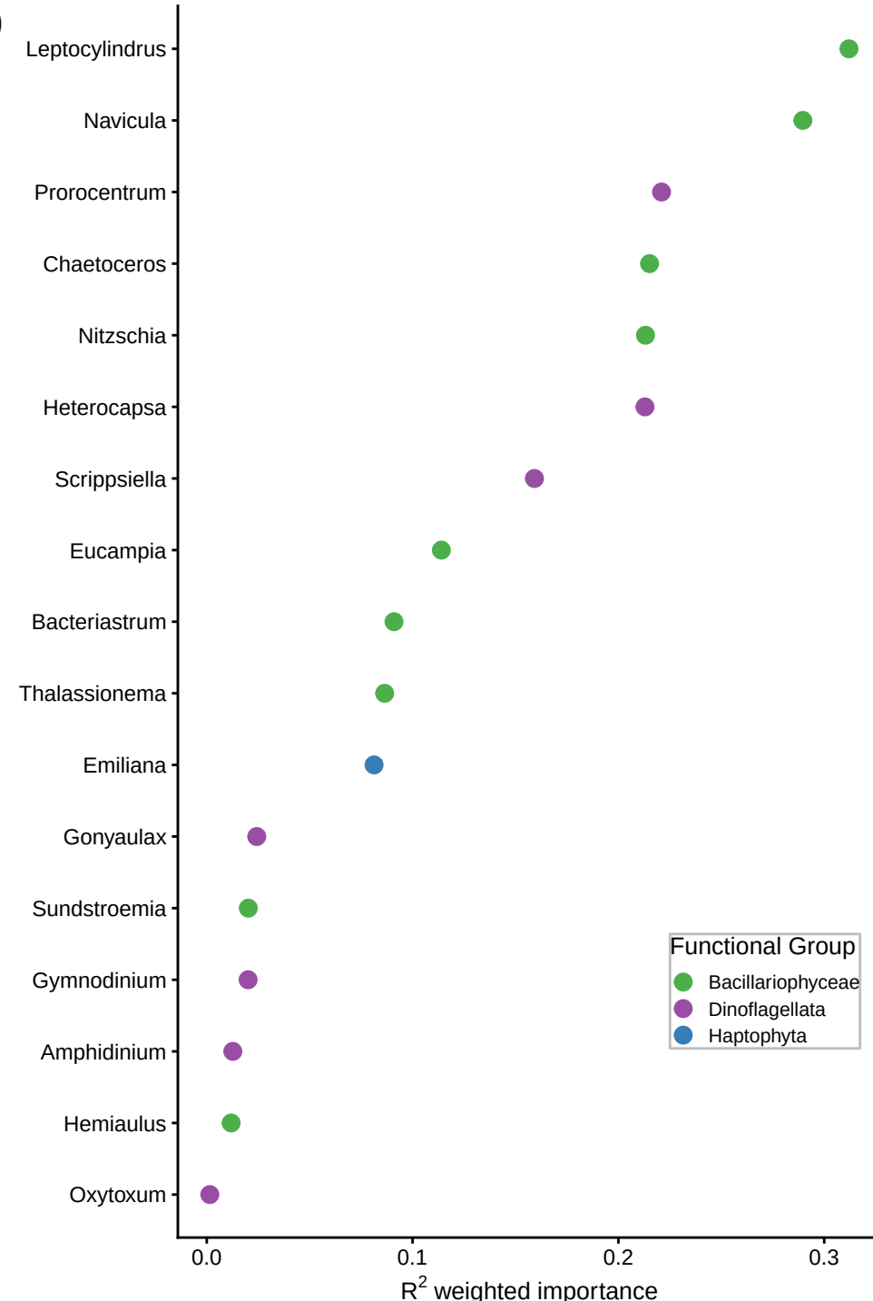
Variable Importance (optimized lags)
