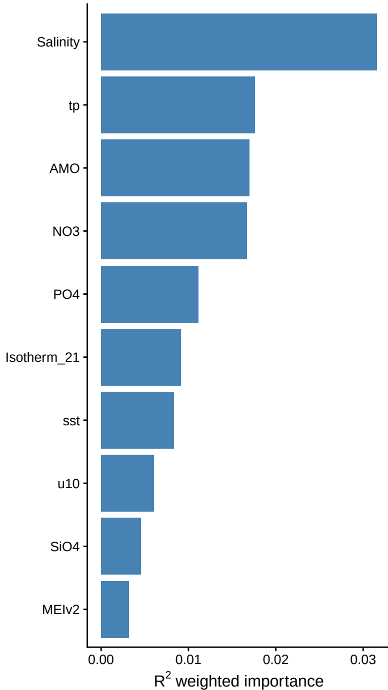
Variable Importance (no lag)
