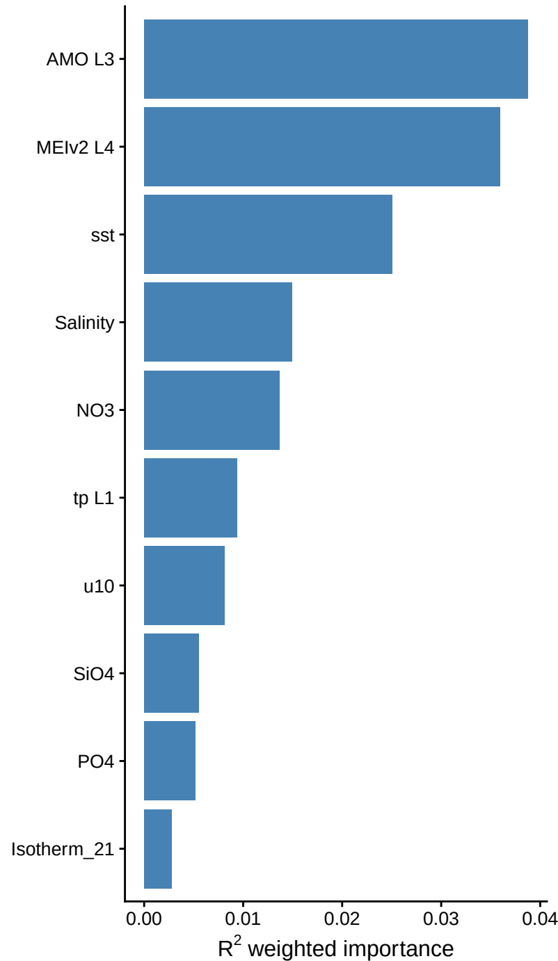
Variable Importance (optimized lags)
