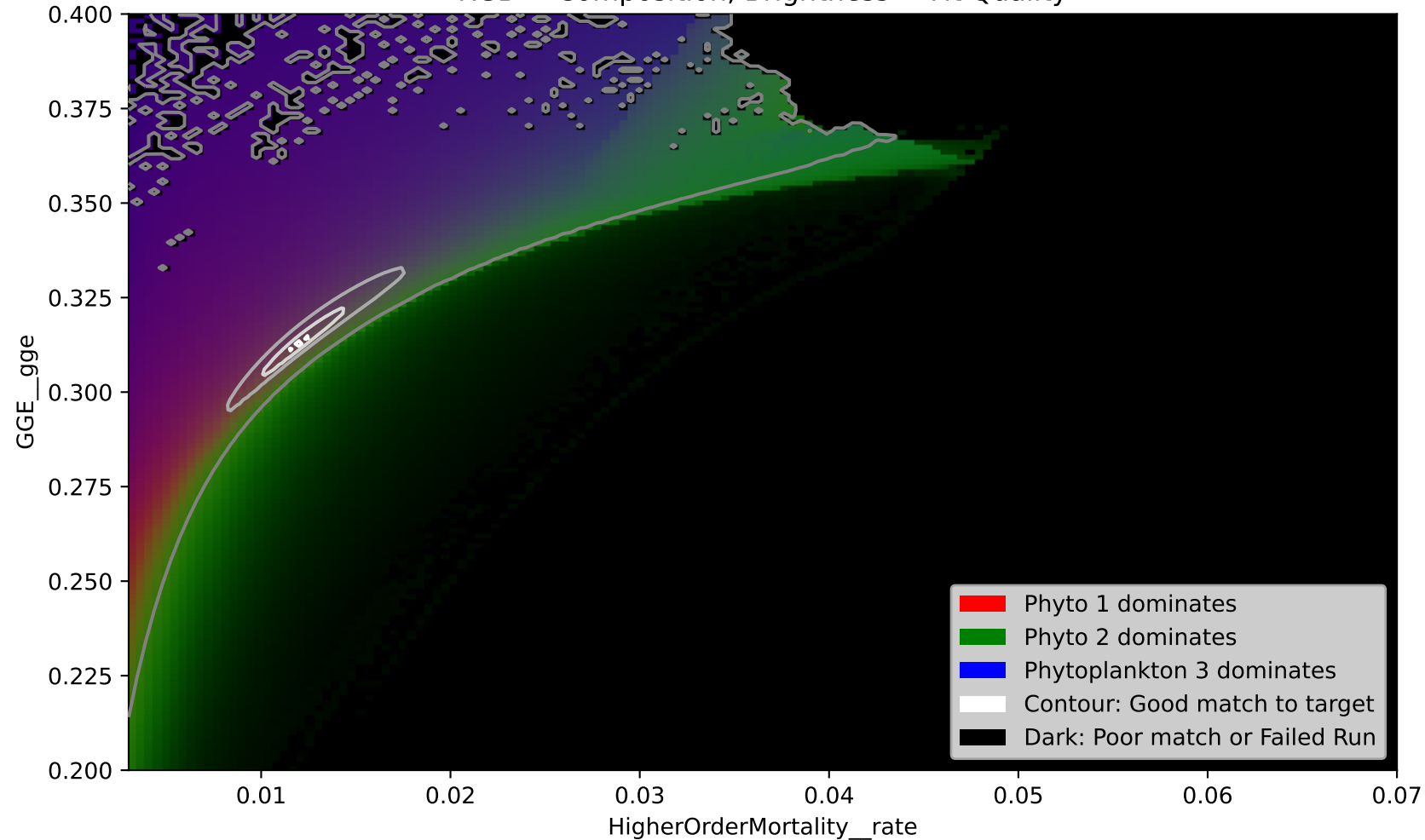
Phytoplankton Composition Fit RGB = Composition, Brightness = Fit Quality
