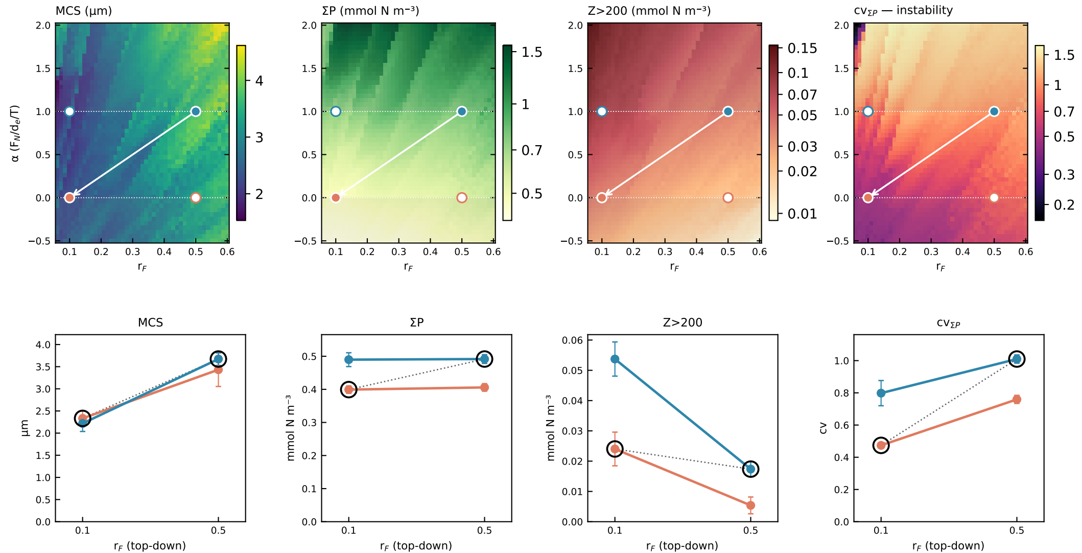
Figure 5 — bottom-up ( \alpha ) \times top-down ( r_F ): landscape (row 1) + 2 \times 2 corner decomposition (row 2) \cdot construct D, idealised \alpha -forcing
