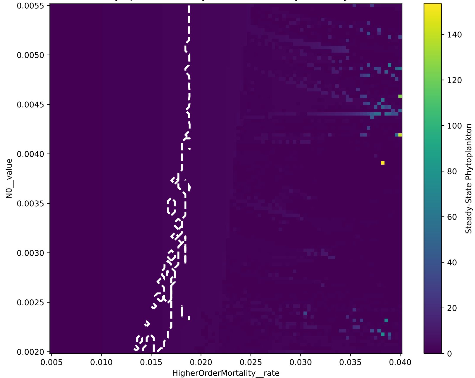
Phytoplankton Steady State with Stability Boundary
