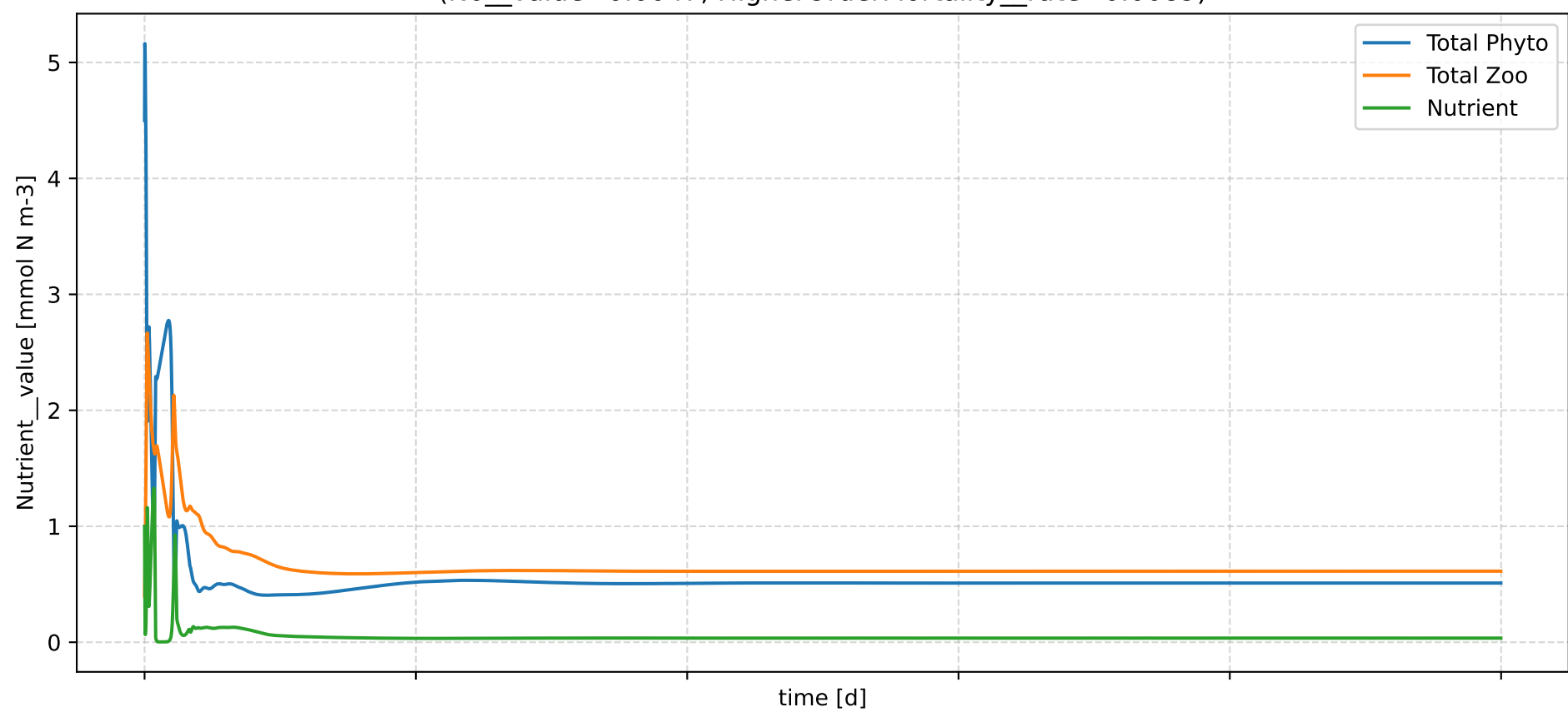
Example 2: Unstable & Meaningful (Likely Oscillations) (N0__value=0.0055, HigherOrderMortality__rate=0.0244)
