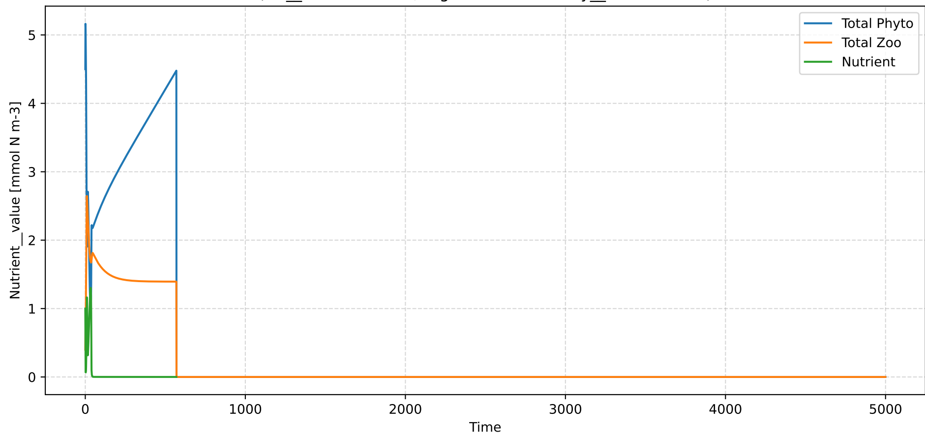
Example 3: Washout / Non-Meaningful (N0__value=0.0039, HigherOrderMortality__rate=0.0400)
