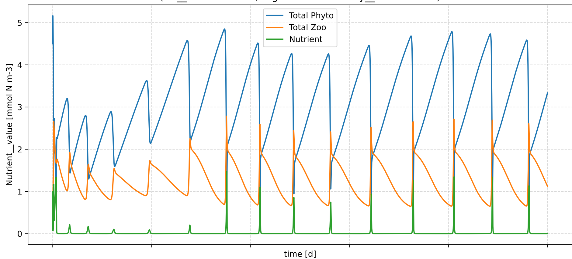
Example 3: Washout / Non-Meaningful (N0__value=0.0039, HigherOrderMortality__rate=0.0400)
