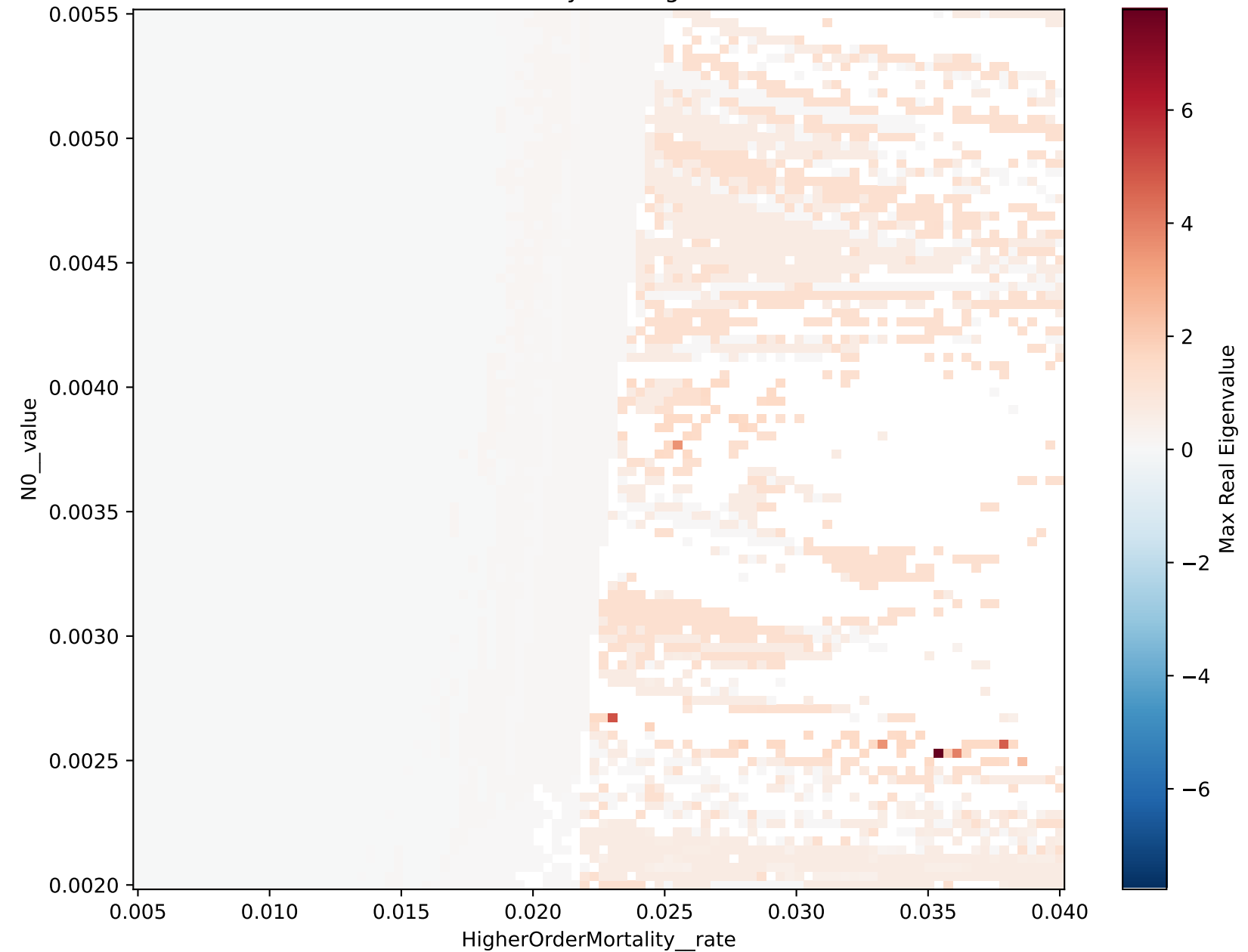
Stability "Strength"
