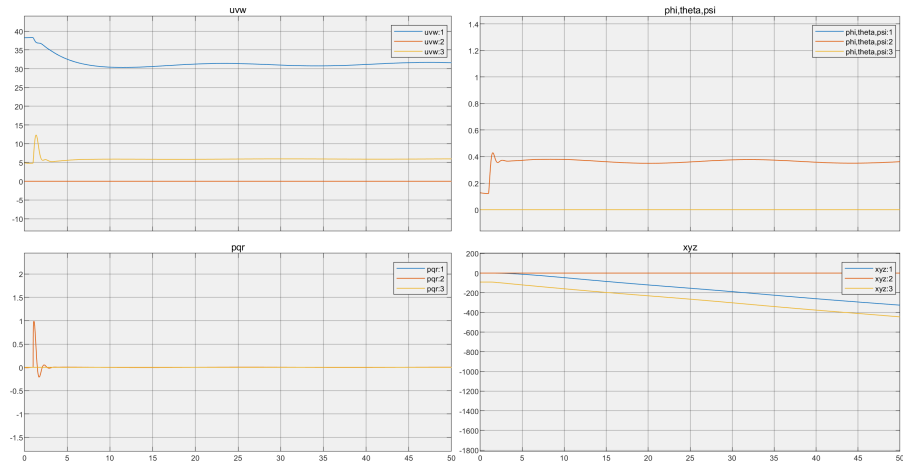
Figure 24: 6 DOF State-Space System Linear Response to Gust
