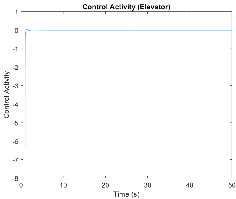
Figure 18: Elevator Control Activity (Auto Throttle System)
