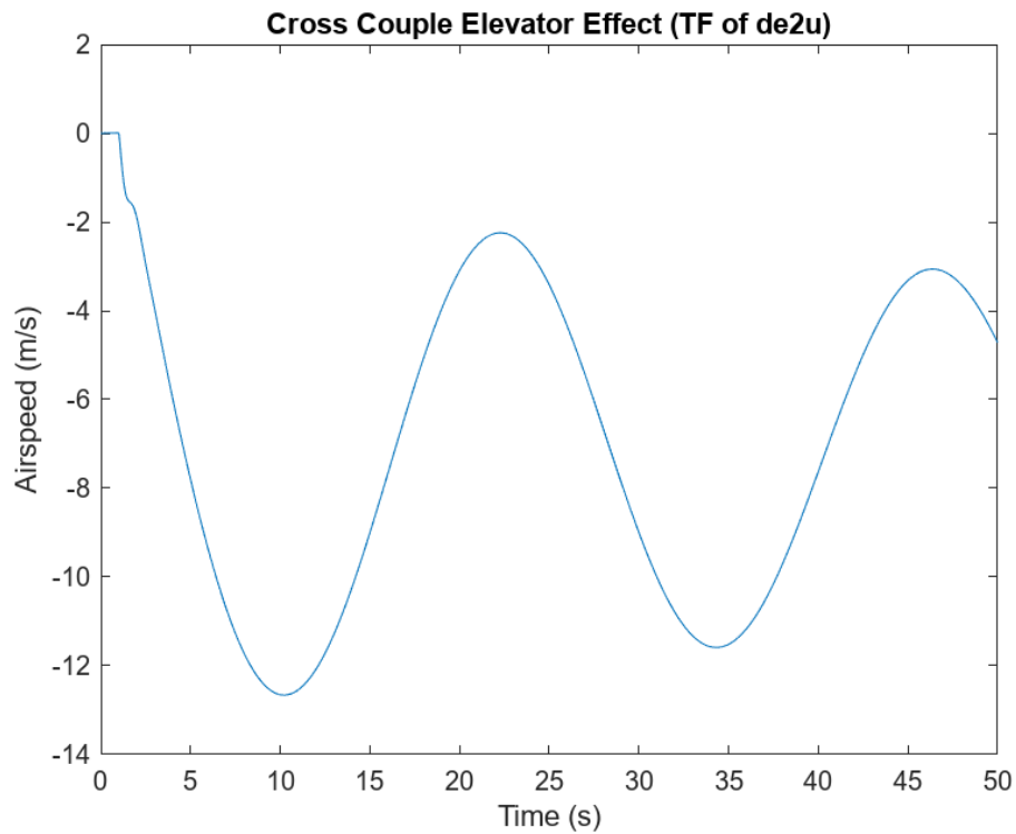
Figure 17: Cross Couple Response (Elevator to Airspeed)
