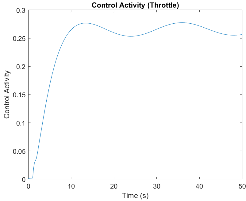
Figure 19: Throttle Control Activity (Auto Throttle System)
