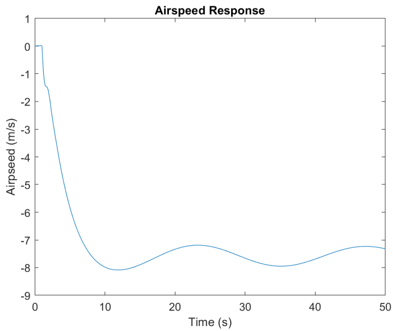
Figure 15: Airspeed Response (Auto Throttle System)
