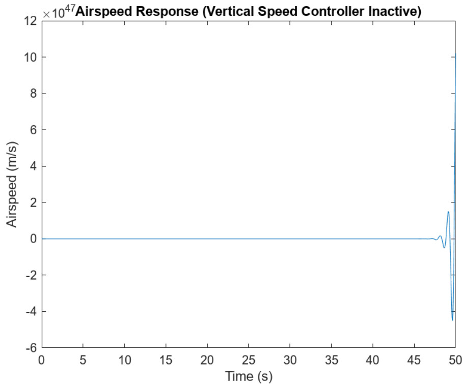
Figure 20: Airspeed Response with Vertical Speed Controller Deactivated
