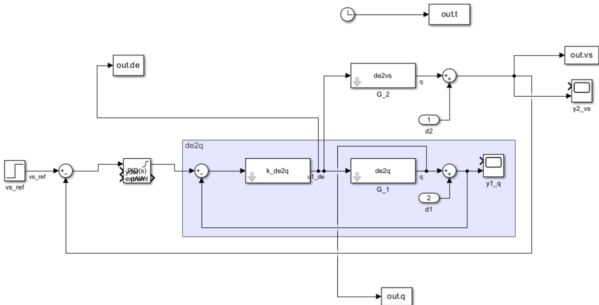
Figure 2: Vertical Speed Guidance Loop Topology
