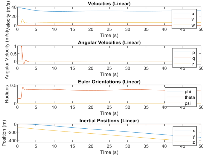
Figure 23: 6 DOF State-Space System Linear Response to Gust
