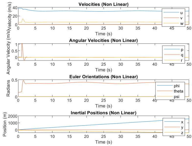
Figure 24: 6 DOF State-Space System Nonlinear Response to Gust
