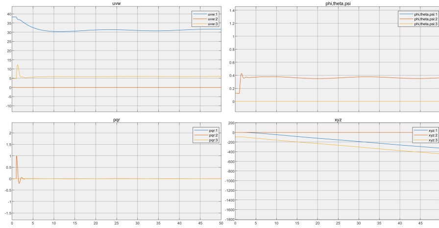
Figure 23: 6 DOF State-Space System Linear Response to Gust
