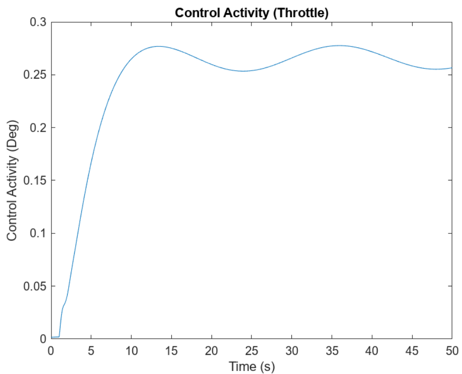
Figure 18: Throttle Control Activity (Auto Throttle System)
