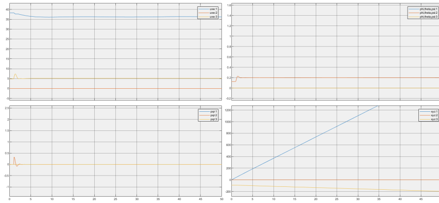
Figure 21: 6 DOF State-Space System Nonlinear Response
