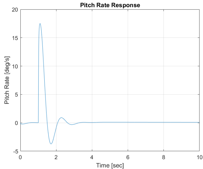
Figure 8: Pitch Rate Response
