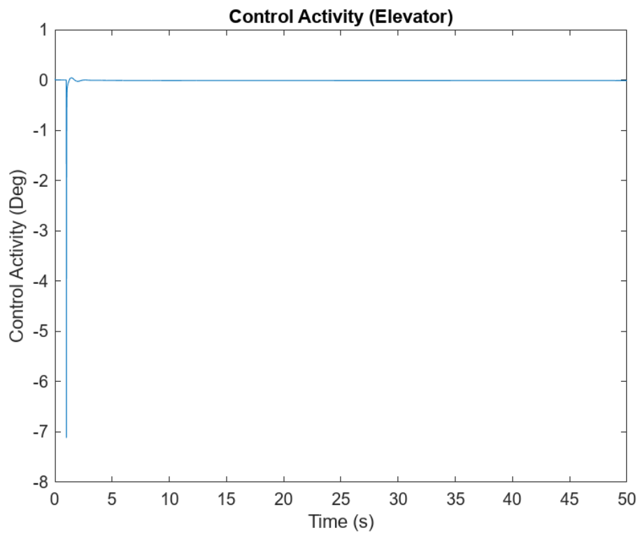
Figure 17: Elevator Control Activity (Auto Throttle System)
