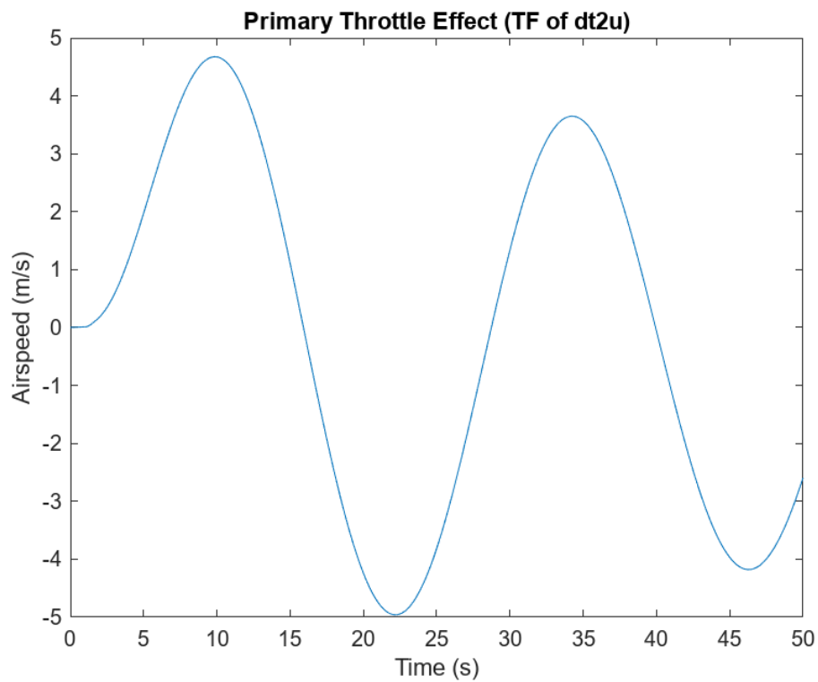
Figure 11: Primary Control Effect: Throttle to Airspeed
