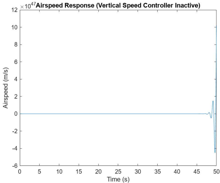
Figure 19: Airspeed Response with Vertical Speed Controller Deactivated
