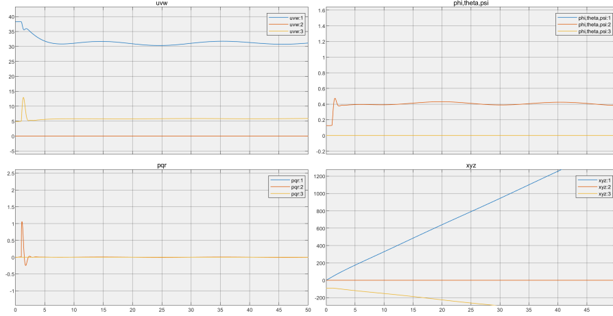
Figure 24: 6 DOF State-Space System Nonlinear Response to Gust
