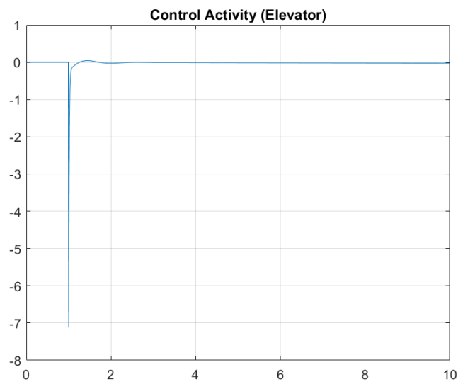
Figure 6: Elevator Control Activity
