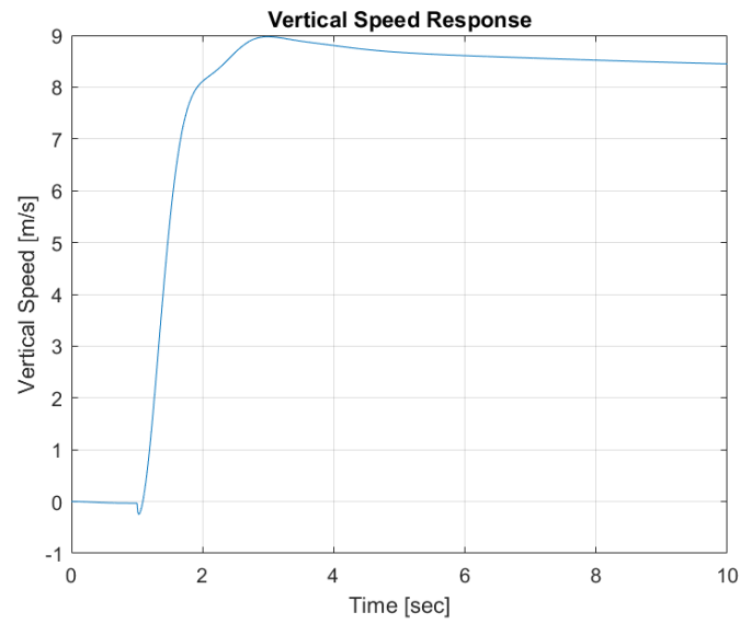
Figure 4: Vertical Speed Response
