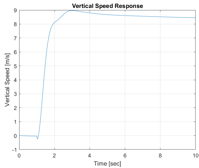
Figure 2: Vertical Speed Response
