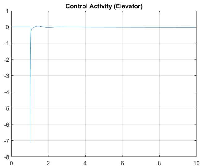
Figure 4: Elevator Control Activity
