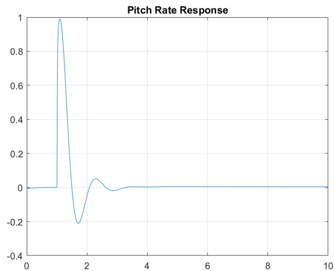
Figure 3: Pitch Rate Response
