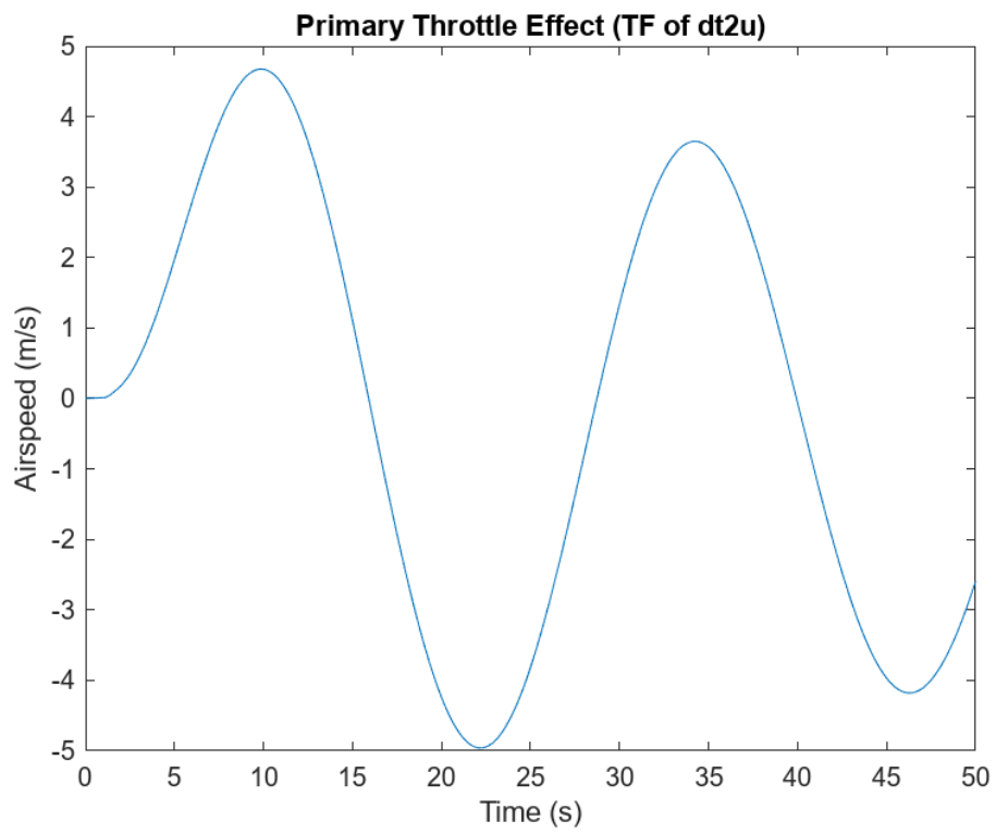
Figure 6: Primary Control Effect: Throttle to Airspeed
