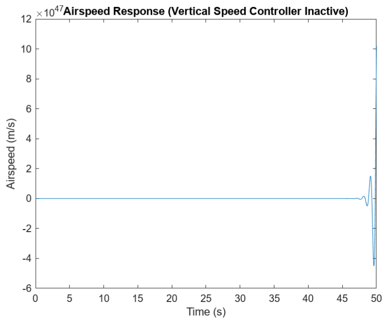
Figure 20: Airspeed Response with Vertical Speed Controller Deactivated
