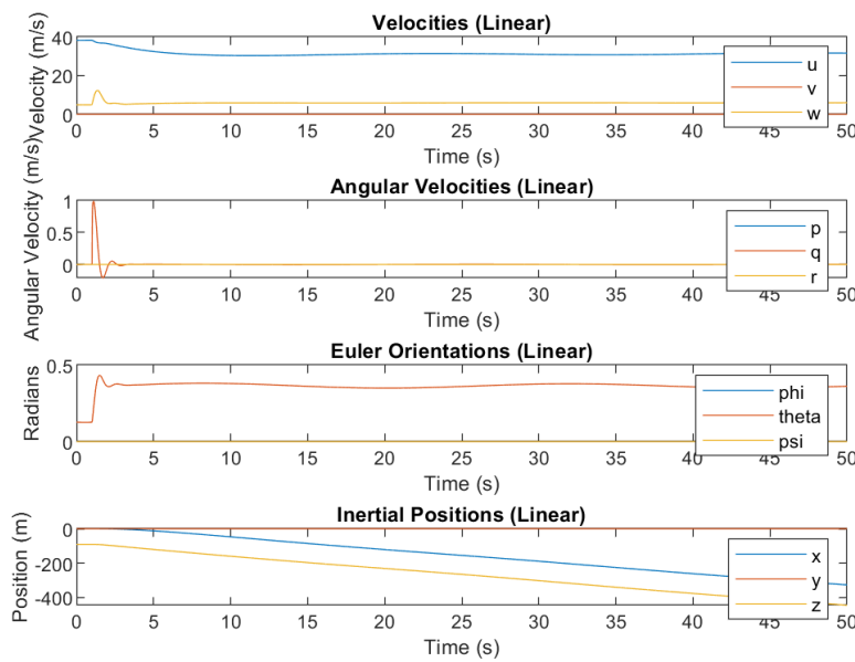
Figure 22: 6 DOF State-Space System Linear Response
