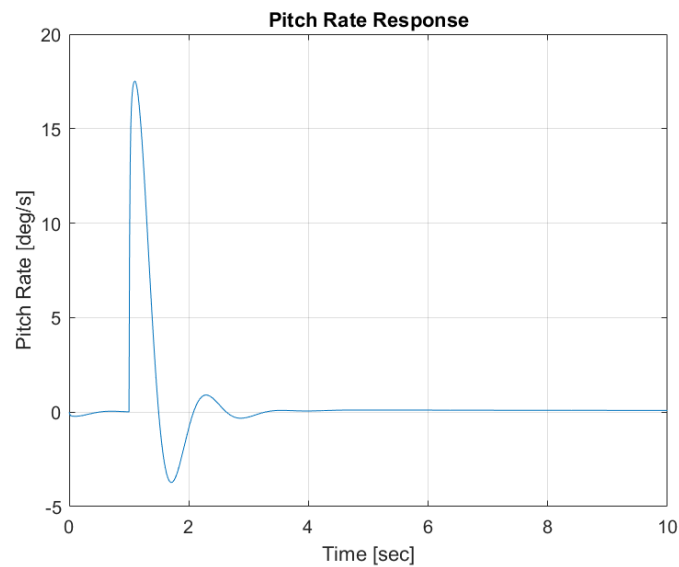
Figure 4: Pitch Rate Response
