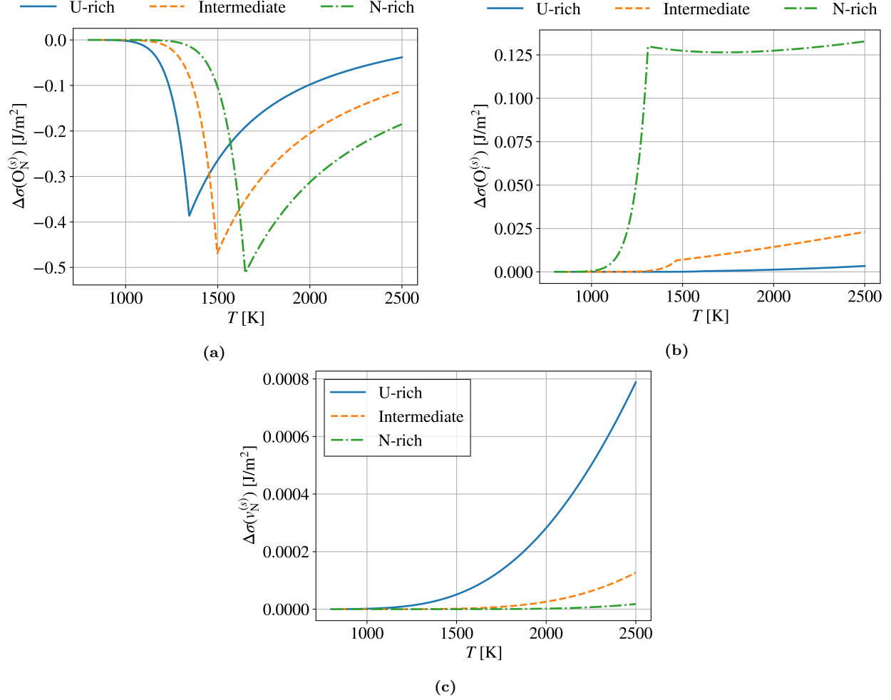
Figure 7: Different terms of the surface energy change due to oxygen adsorption and vacancy formation on void surfaces for w_O = 1500 ppm, p = 5\% , and R_v = 1 nm. (a) \Delta\sigma(O_N^{(s)}) , (b) \Delta\sigma(O_i^{(s)}) , and (c) \Delta\sigma(v_N^{(s)}) are given in Eqs. (34) to (36), respectively.
