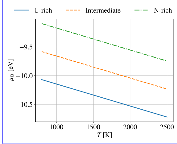
Figure 2: Oxygen chemical potential as calculated based on Eq. (16).
