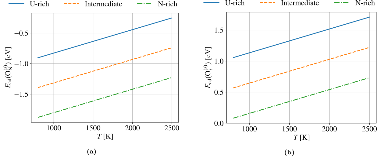
Figure 3: Temperature evolution of oxygen adsorption energy relative to the chemical potential shown in Fig. 2 for (a) \text{O}_\text{N}^{(\text{s})} and (b) \text{O}_\text{i}^{(\text{s})} .
