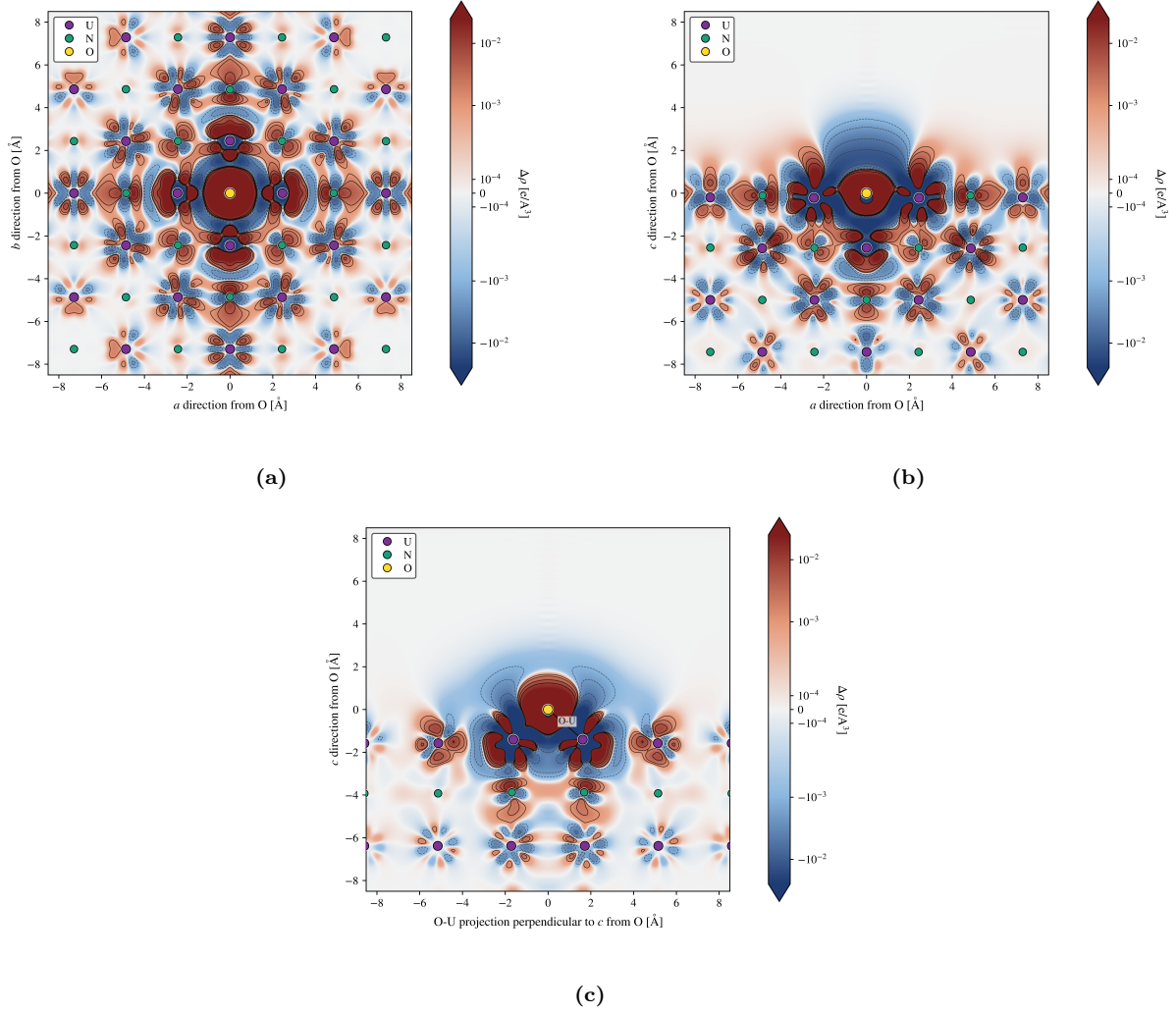
Figure 4: Charge-density difference, \Delta\rho , around surface oxygen in UN. (a) \text{O}_\text{N}^{(\text{s})} in the a - b plane. (b) \text{O}_\text{N}^{(\text{s})} in the a - c plane. (c) \text{O}_\text{i}^{(\text{s})} in the plane spanned by the nearest O-U direction and the crystallographic c axis, with c vertical. Red denotes electron accumulation and blue denotes electron depletion in \Delta\rho . Solid and dashed contours mark positive and negative \Delta\rho , respectively. U, N, and O atoms are shown as purple, green, and yellow markers.
