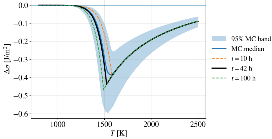
Figure F.12: Correlated Monte Carlo uncertainty band for \Delta\sigma(T) at the reference case. The shaded region is the 2.5–97.5 percentile range, the solid curve is the Monte Carlo median, and the baseline curves show the deterministic model at t = 10, 42 , and 100 h. The energetic uncertainty is bounded by \pm 0.1 eV, with shared systematic shifts applied to the oxygen-related and vacancy-related energy pairs. The migration energy E_m is also varied and is updated consistently in both the Arrhenius exponent and the attempt-frequency prefactor.
