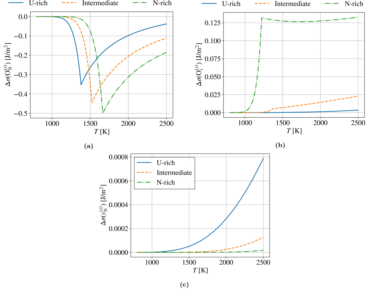
Figure 8: Different terms of the surface energy change due to oxygen adsorption and vacancy formation on void surfaces for w_O = 1500 ppm, p = 5\% , and R_v = 1 nm. (a) \Delta\sigma(O_N^{(s)}) , (b) \Delta\sigma(O_i^{(s)}) , and (c) \Delta\sigma(v_N^{(s)}) are given in Eqs. (36) to (38), respectively.
