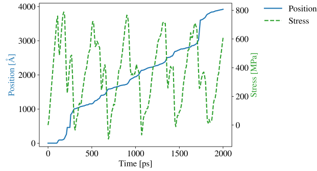
Figure 7. Movement of the \frac{1}{2}\langle 110 \rangle \{110\} screw dislocation at 1 K under an applied strain rate of 10^{-4} \text{ s}^{-1} as predicted by the Kocevski potential. The average of the developed \sigma_{yz} stress on the dislocation is also shown.
